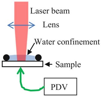
Fig. 2.6 Left: Experimental setup of laser shock wave on UHMWPE. Center: trace of impact resulting from the laser-matter interaction. Right: visible bulge at the free surface
