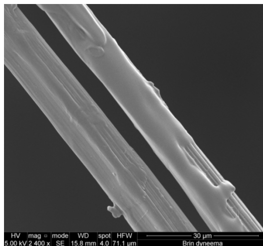
Figure 14. Two SK99 filaments
