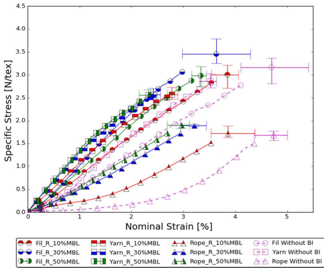
Figure 13.e. Tension after Relaxation BI
