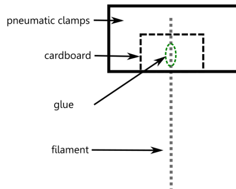
Figure 8. Attachment method for filament samples.
