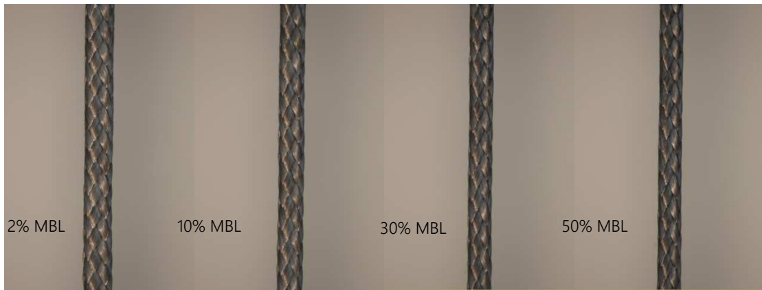
Figure 16. Images of the evolution of the rope's width during tension loading for Dyneema SK99 rope with a diameter of 4mm
