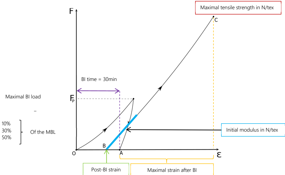
Figure 9. Extracted data for the case of load/unload bedding-in (BI) protocol.
