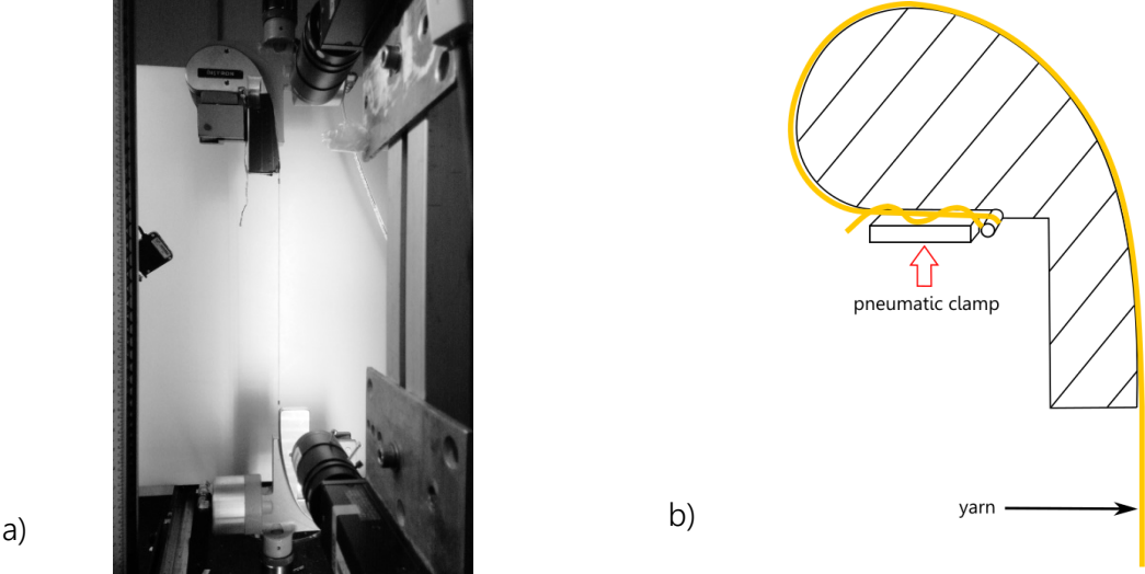
Figure 7. Yarn sample on test machine (a) and attachment method (b).
