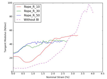
Figure 21.c. Change in tangent modulus for R BI protocol
