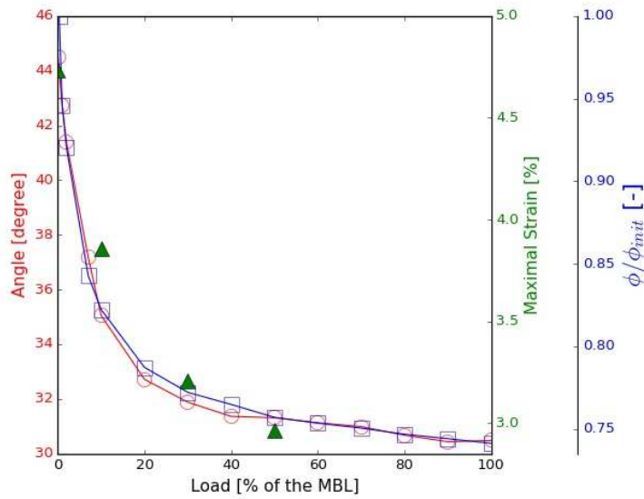
Figure 19. Evolution of the maximal strain after BI at different load levels (triangle), the apparent diameter (square) and the evolution of the angle between strands with loading (circle).
