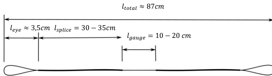
Figure 3. Rope sample geometry.
