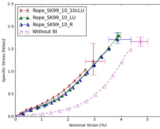
Figure 12. a. Rope results for a maximal BI load of 10% of the MBL.
