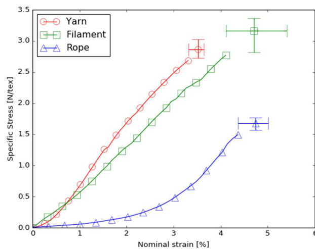
Figure 11. Monotonous loading without BI for each scale of the rope
