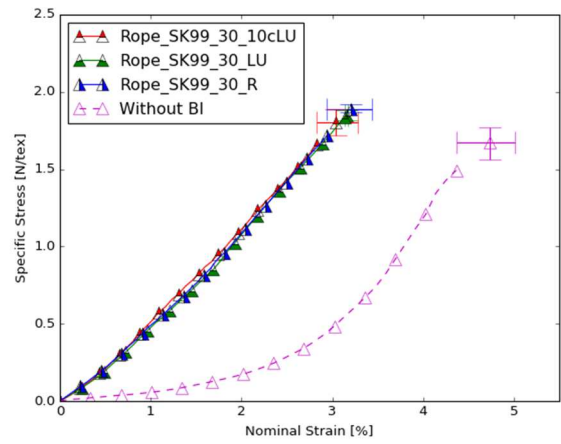
Figure 12. b. Rope results for a maximal BI load of 30% of the MBL.
