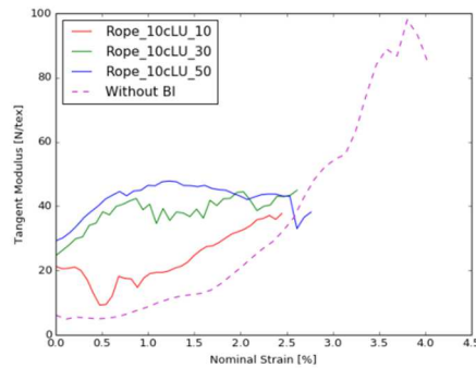
Figure 21.b. Change in tangent modulus for 10cLU BI protocol
