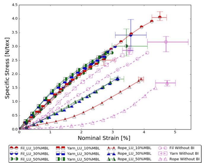
Figure 13.d. Tension after Load-Unload BI
