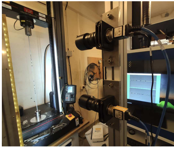
Figure 4. Monotonous loading on rope with different markers
