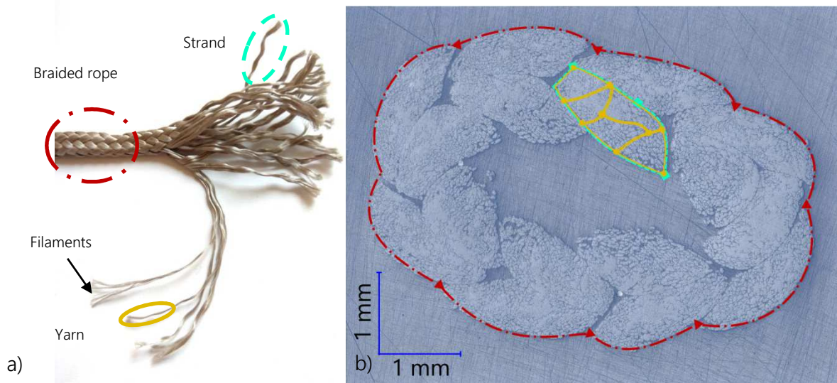
Figure 1. a) The studied braided rope and its components, b) section through new rope before loading, showing strands, yarns and filaments.
