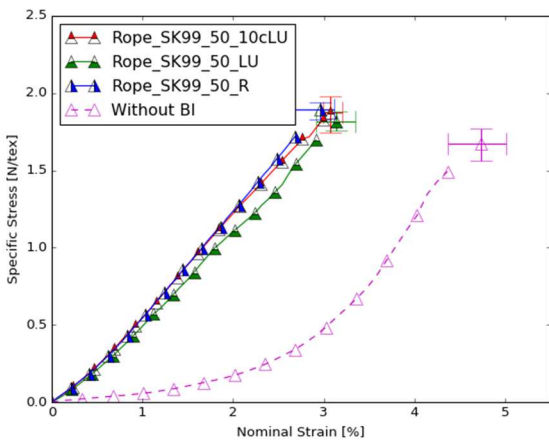
Figure 12. c. Rope results for a maximal BI load of 50% of the MBL.
