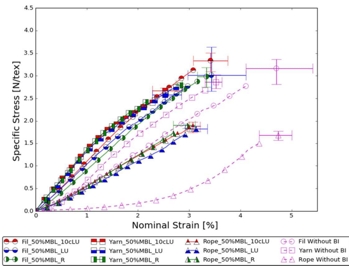
Figure 13.c. Tension after 50%MBL BI
