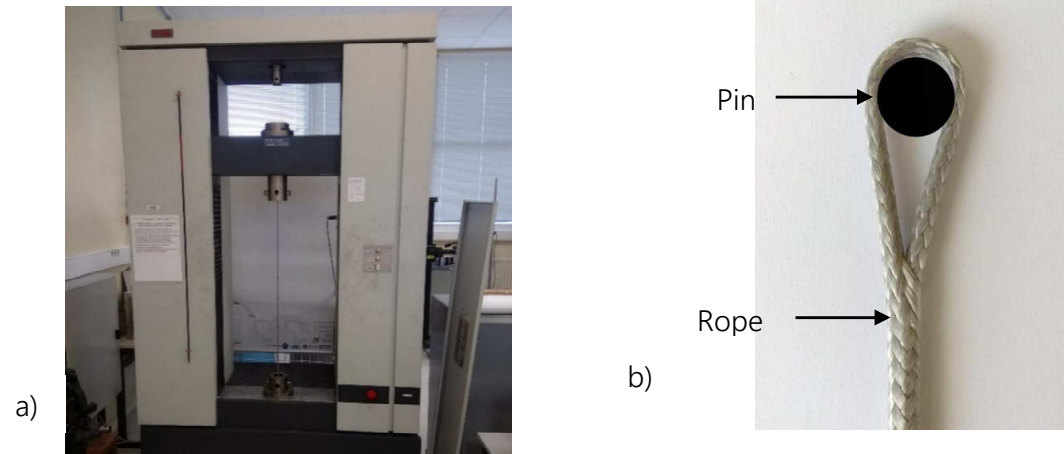
Figure 2. a) Rope sample on test machine and b) attachment method by splice.
