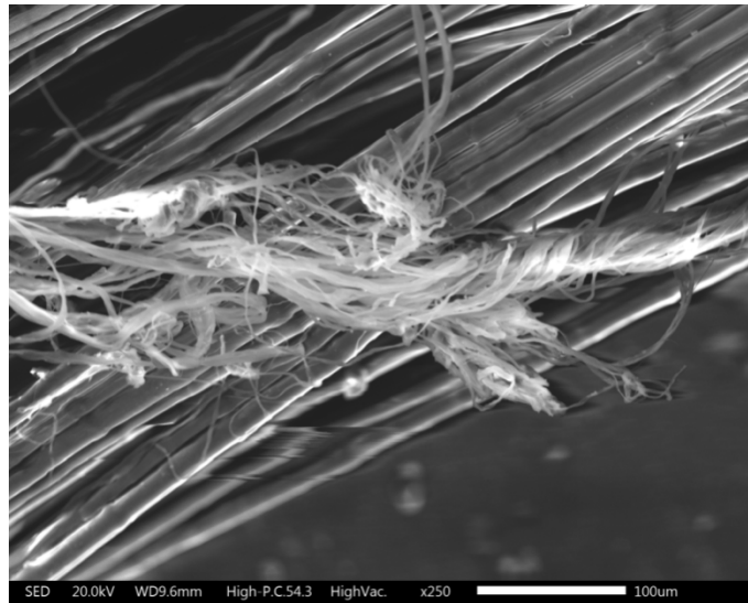
Figure 15. SEM image of extracted Dyneema filaments
