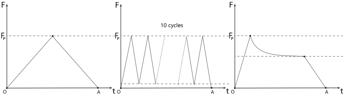
Figure 10. Bedding-in protocols studied
