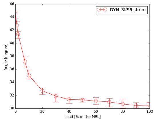
Figure 18. Change in the angle \alpha between strands during tension loading for Dyneema SK99 rope with a diameter of 4mm. The error bars correspond to the minimum and the maximum angle measurements.
