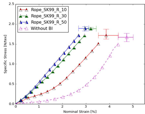
Figure 12. d. Rope results: comparison between a maximal BI load of 10%, 30% and 50% for Relaxation BI.
