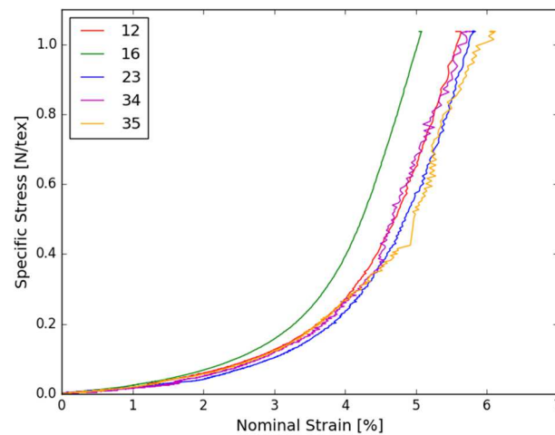
Figure 6. Stress-Strain results for different markers
