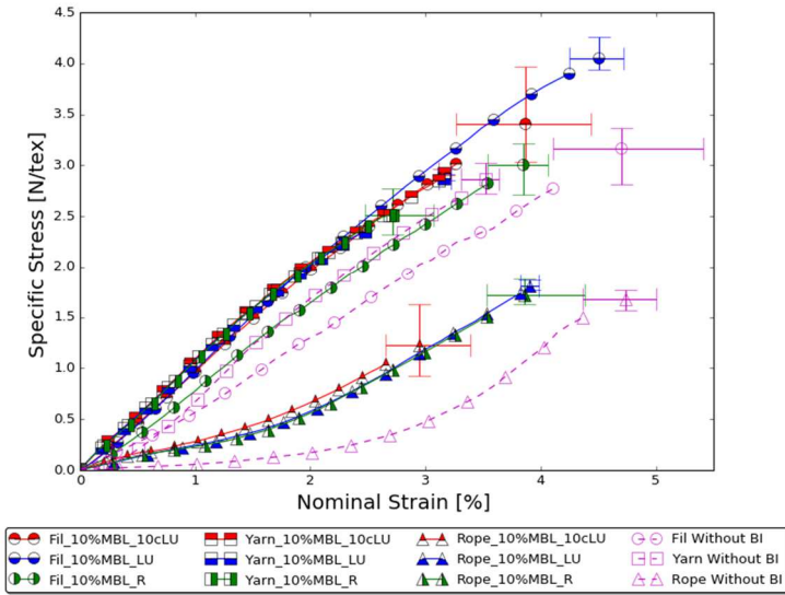
Figure 13.a. Tension after 10%MBL BI
