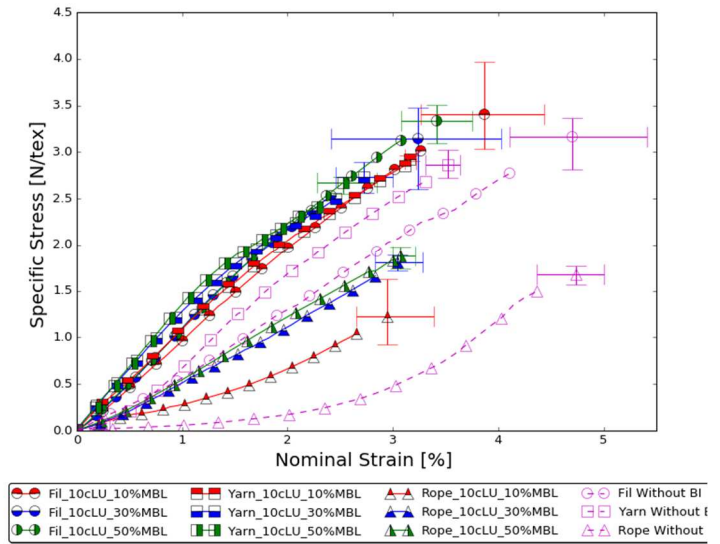
Figure 13.f. Tension after 10 load/unload cycles BI
