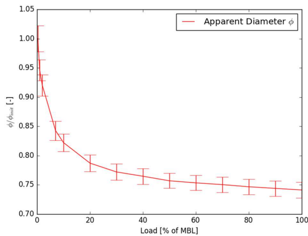
Figure 17. Change in the apparent diameter with tension loading. Error bars show standard deviation.
