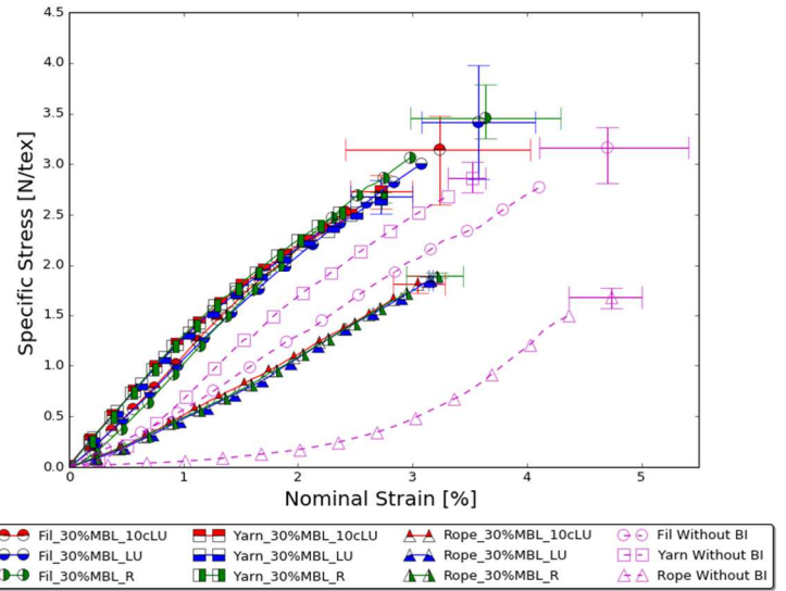
Figure 13.b. Tension after 30%MBL BI
