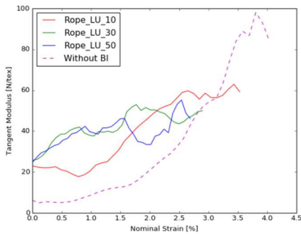
Figure 21.a. Change in tangent modulus for LU BI protocol
