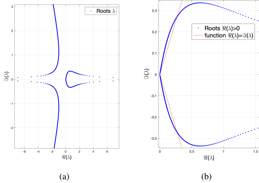
Figure 5.1: Evolution of the four roots \lambda_i in the complex plane, as a function of \mu . (a): global picture with 4 trajectories. (b): zoom in the right-half plane \Re(\sigma) > 0 , 2 trajectories crossing the segment \Re(\lambda) = |\Im(\lambda)| for a critical value \mu^c of the viscosity.
