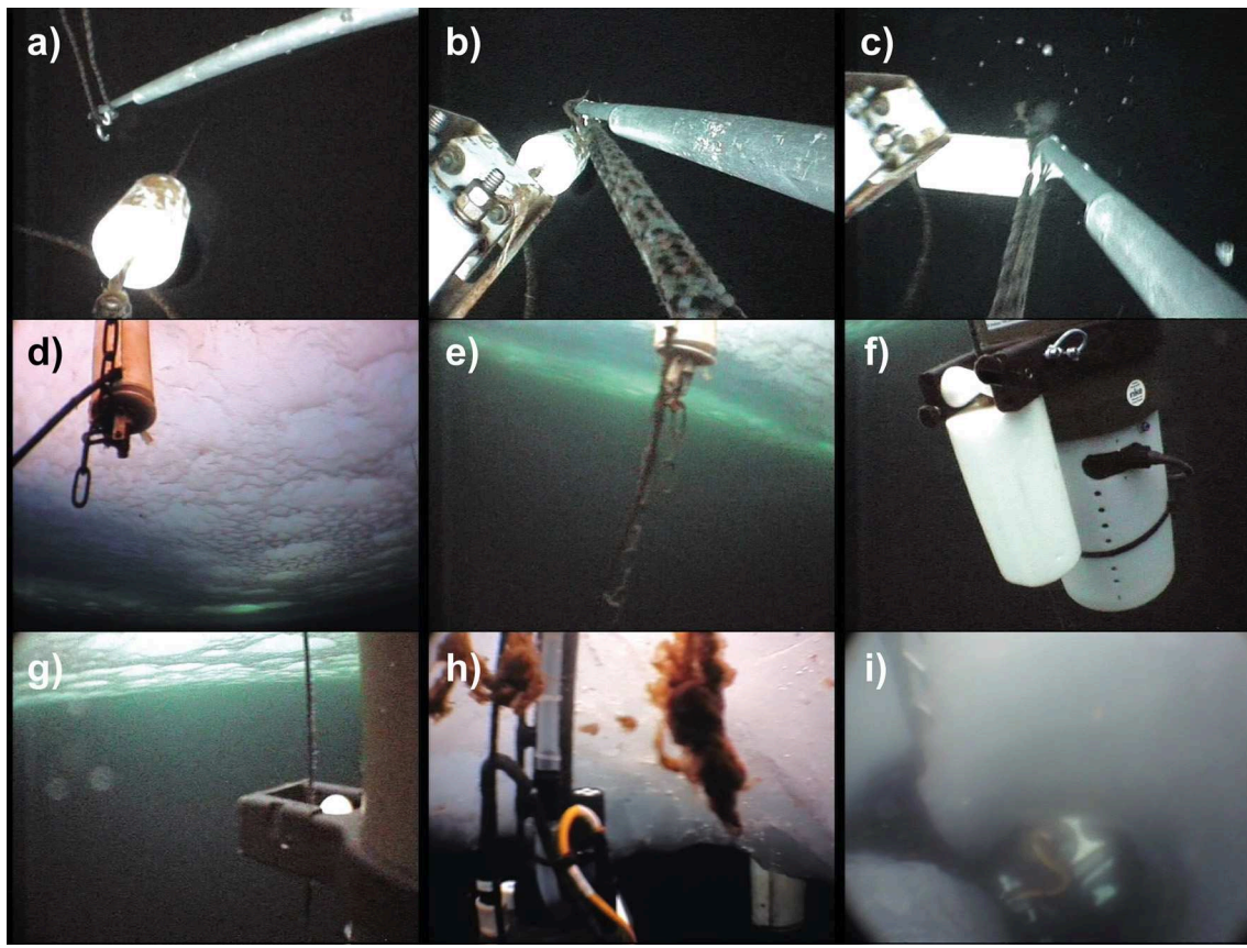
FIGURE 3 | Screenshots taken from the underwater camera during recovery work: (a) Clipping a biner with rope loop into the wire below the top stop. (b) After the biner is clipped into the wire. (c) Taking the load onto the initial recovery system. (d) The attachment chain is fully stretched and pointing upwards, while the umbilical leading to the inductive modem was already cut. (e) After removal of the wire and inductive modem, the chain, and umbilical hang down straight again. (f) Profiler resting on the bottom stop during recovery. (g) Profiler attachment to wire, note the algal contamination on wire. (h) profiler underneath the recovery hole. The floating algal flocks result from biofouling on the wire stripped off by the friction knot. (i) Removing the last ice nose prohibiting profiler recovery with the ice saw (top left image corner). The bright white buoyancy pack of the profiler is already visible under the hole.
