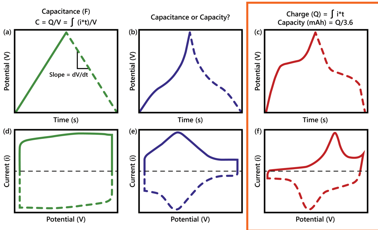
Figure 1. Archetypal electrical output behavior of three main types of electrodes, including a, d) electrical double layer, b, e) pseudocapacitive, and c, f) battery type. a–c) Schematic of galvanostatic charge-discharge profiles showing linear and nonlinear responses with time and d–f) corresponding CV profiles.
