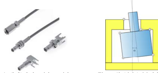
Fig. 1a (left): Industrial coaxial connector. Figure 1b (right): Model of the considered mechanism with gaps. Gaps are emphasized for a better comprehension.
