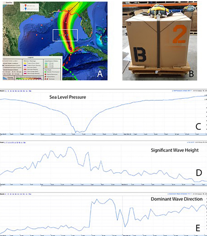
FIGURE 5 | (A) Deployment location of 10 drifters ahead of Hurricane Michael (white box). The drifters were deployed on October 8, 2018, from a C-130J aircraft by the United States Air Force Reserve's 53rd Weather Reconnaissance Squadron "Hurricane Hunters." The transect was located approximately 24 h ahead of the predicted track of the storm, which is shown by green and red symbols. The forecast for the wind intensity is overlaid as a contour plot (see legend in panel A ). The storm data were provided by NOAA's National Hurricane Center (NHC). The 10 drifters were air-deployed at five stations using the deployment package shown in panel (B) . Each box contained one SVP-B drifter and one directional wave spectra (DWS) drifter. One SVP-B drifter measured a minimum air pressure of 967.7 hPa inside the eye of the hurricane (C) . The DWS drifter deployed at the same location measured a maximum significant wave height of 8.7 m (D) . Note the sharp change of the dominant wave direction due to the hurricane moving over the DWS drifter (E) and the rapid decay of the wave field in the wake of the storm.
