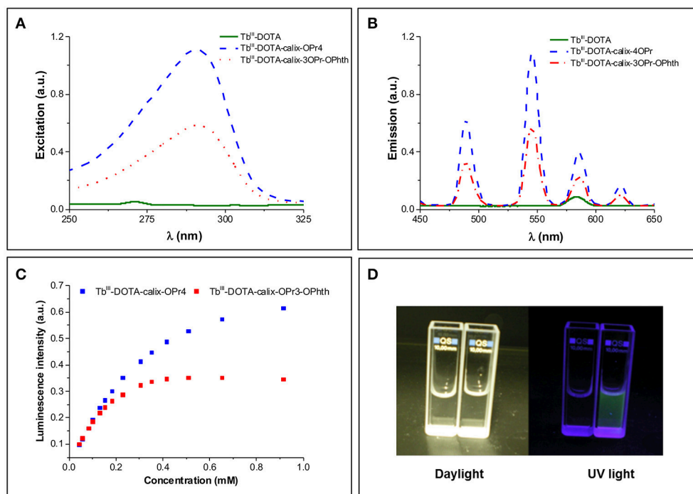
FIGURE 3 | (A) Excitation ( \lambda_{Em} = 545 nm) and (B) emission ( \lambda_{Ex} = 290 nm) spectra of Tb^{III} -DOTA, Tb-12a and Tb-12b at a Tb^{III} concentration of 3.68 mM (corresponding to a calix[4]arene concentration of 0.92 mM). The two little signals at 272 nm (excitation) and 580 nm (emission) in the Tb^{III} -DOTA spectra are artifacts from light scattering (double wavelength of excitation); (C) The dependence of relative luminescence intensities normalized to the same initial value vs. the concentration of Tb-12a and Tb-12b ; (D) Photographic images of Tb^{III} -DOTA (left cuvette) and Tb-12a (right cuvette) under daylight and UV irradiation.
