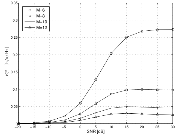
Fig. 4: E_s^m vs. the transmit SNR \rho , in the presence of an external eavesdropper.
