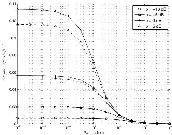
Fig. 6: E_s^m and \hat{E}_s^m vs. the delay exponent \theta_m , for different values of \rho , with an external eavesdropper.
