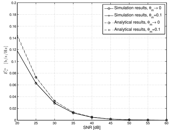
Fig. 7: E_s^m vs. the transmit SNR \rho , for different \theta_m values, with an external eavesdropper.
