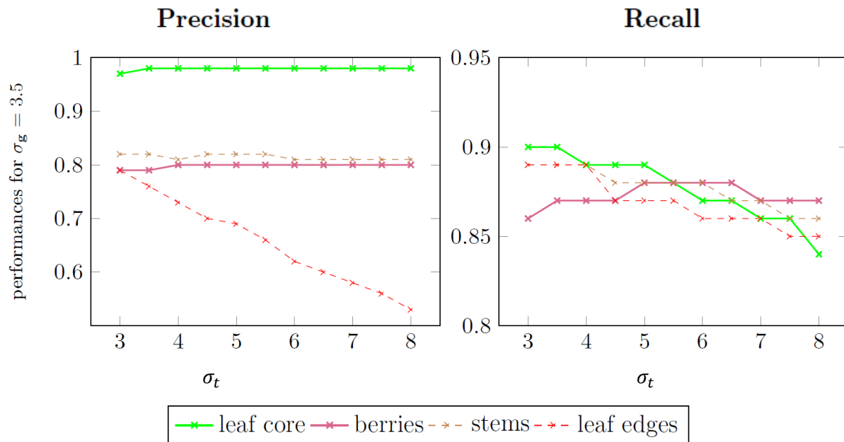
Figure 3 - Influence of \sigma_t scale for optimal value of \sigma_g on precision and recall metrics for stage BBCH 79
