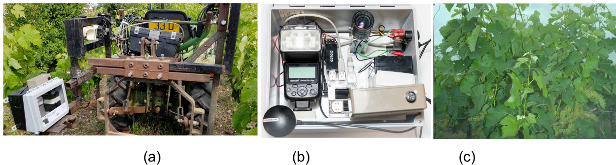
Figure 1- Instrumentation: embedding on a vineyard tractor (a), device compounds (b) and example of a resulting image (c)
