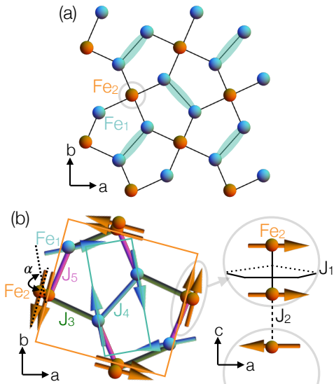
FIG. 1. (a) ab plane projection of the Fe atoms in \text{Bi}_2\text{Fe}_4\text{O}_9 forming an equivalent of the Cairo pentagonal lattice. The Fe 1 (in blue) and Fe 2 (in orange) have a different connectivity. Blue ellipses underline strongly coupled antiferromagnetic Fe 1 spins. (b) Magnetic arrangement stabilized below T_N : the orange and blue rectangles materialize the two sets of orthogonal antiferromagnetic pairs in the ab plane [12]. The Fe 2 form ferromagnetic pairs sandwiching the Fe 1 planes. The five exchange interactions within and between the pentagonal planes are labeled.
