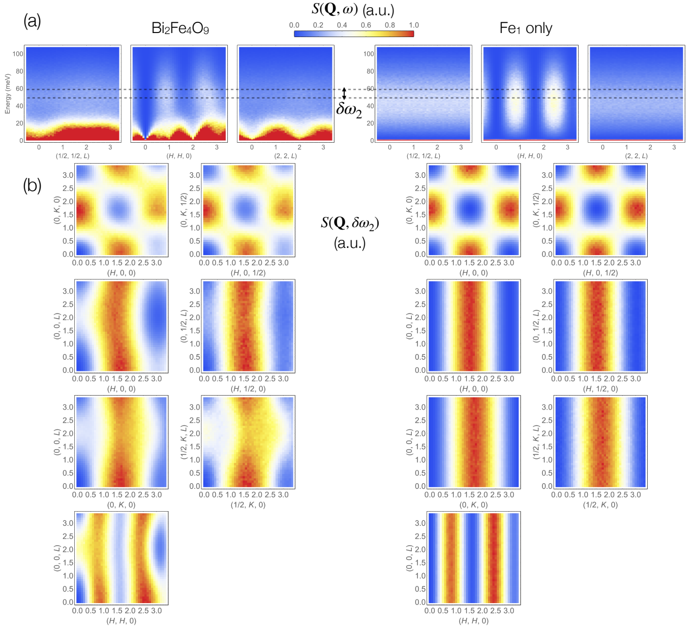
FIG. S9. Comparison of the calculated S(\mathbf{Q}, \omega) for Bi 2 Fe 4 O 9 using the set of exchange coupling obtained from our spin waves analysis with the one taking into account only the Fe_1 spins coupled via J_4 , at T/T_N \simeq 7 through (a) Q-cuts and (b) constant \omega -cuts over an energy range \delta\omega_2 (between the dotted lines). The intensity scale is the same for all the (a) maps and varies for the (b) maps in order to emphasize the main features.
