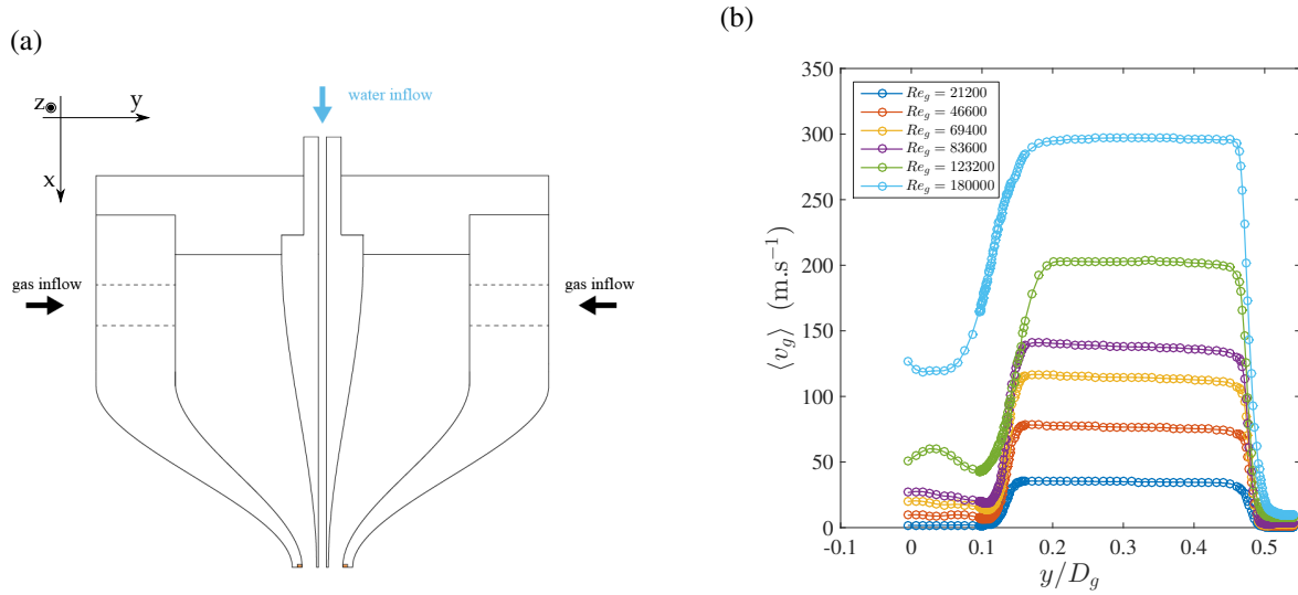
Figure 1. The Canonical Atomizer. (a) CAD drawing of the Canonical Atomizer. (b) Boundary layer measurements collected using Hot-Wire Anemometry 0.25 mm downstream of the nozzle exit, over a wide range of Reynolds numbers.
