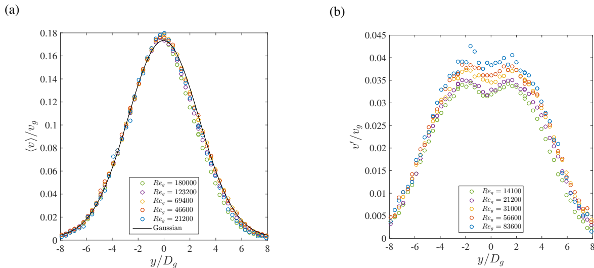
Figure 2. Far-field ( x/D_g = 30 ) gas phase velocity profiles where the velocity has been decomposed into a mean and fluctuating part: v_g = \langle v_g \rangle + v'_g . M = [5, 25, 80, 174, 370] . (a) Mean field velocity ( \langle v_g \rangle ) profiles are self-similar in the far-field and well approximated by a Gaussian curve. (b) Fluctuating ( v'_g ) velocity are nearly self-similar in the far-field, though the collapse is only partial for the lowest Reynolds numbers.
