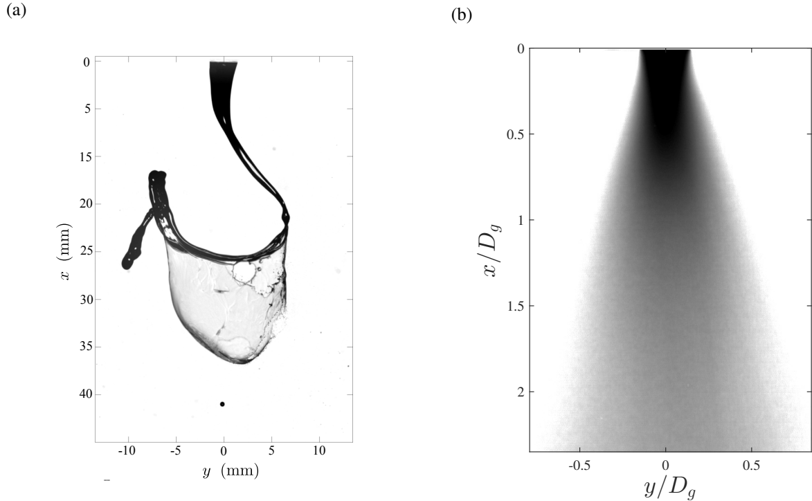
Figure 3. Shadowgraph images. (a) High speed image using the Shadowgraph technique of at Re_g = 10600 and M = 1.1 . (b) Average pixel intensity \langle I \rangle of images from the Re_g = 31000 and M = 11 . The average pixel intensity is related to the probability that the liquid phase is present at a given point in the image with the white background indicating low probability and dark regions indicating a high probability of the finding the liquid phase present.
