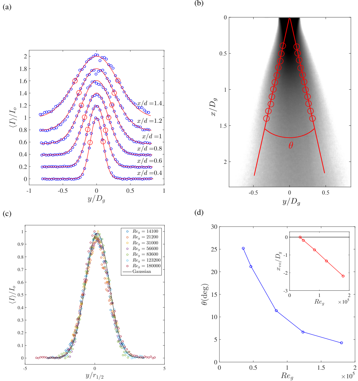
Figure 4. Topological investigation of the liquid-gas phase jet. (a) Normalized pixel intensity profiles ( \circ ) are represented with several transverse Gaussian profiles of the normalized pixel intensity \langle I \rangle / I_o superimposed (red curves). Each profile passes through two circles representing a two standard deviation width. Re_g = 31000 and M = 11 . (b) The increasing values of the transverse standard deviation of normalized average pixel intensity is used to define the opening angle \theta by linear extrapolation. The virtual origin of the liquid-gas phase jet is defined as the point at which the two linear profiles cross. (c) Normalized pixel intensity curves at x/D_g = 2.3 for several different Reynolds numbers. The spatial parameter r_{1/2} refers to the position at which \langle I \rangle / I_o = 0.5 . The black line is a Gaussian fit. The corresponding momentum fluxes are: M = [2, 5, 11, 25, 80, 174, 370] (d) The opening angle \theta is a decreasing function of the Reynolds number. The corresponding momentum fluxes are M = [11, 25, 80, 174, 370] . (d, inset) As the Reynolds number increases the virtual origin moves from the near field of the jet to the interior of the atomizer. A critical Reynolds number Re_g = 31000 occurs where the virtual origin is at the atomizer.
