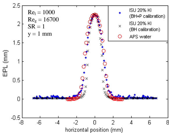
Figure 12: EPL at y = 1 mm below the nozzle, and SR = 1 .
