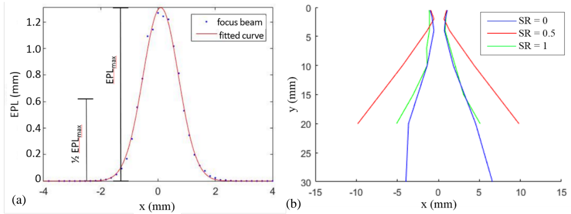
Figure 6: Defining and comparing spray angles for the spray at the flow condition Re_1 = 1,000 and Re_g = 16,700 : (a) Defining \frac{1}{2} EPL_{max} (b) Pinching location moves closer to the nozzle for SR = 0.5 and the spray angle is the largest at this flow condition.
