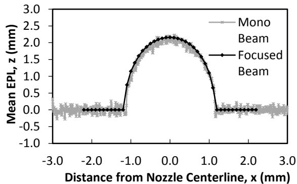
Figure 8 The mean EPL through the laminar water stream ( Re_l = 1000 , Re_g = 0 ) at 0.5 mm downstream from the nozzle exit.
