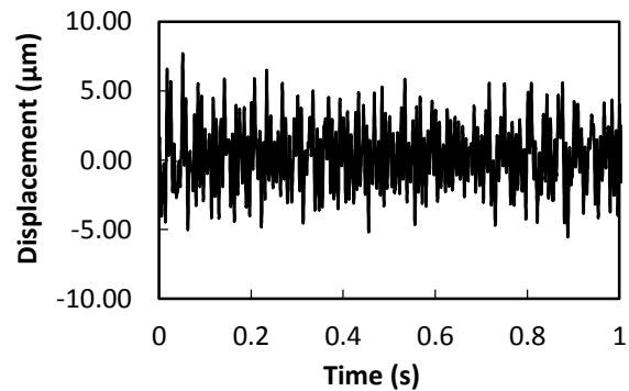
Figure 3 The approximate vertical displacement of the background intensity due to vibrations in the monochromator.
