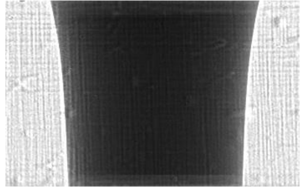
Figure 5 Mono beam image of a laminar liquid stream with Re_l = 1000 . The top of the image corresponds to the nozzle exit and spans a width of 3.4 mm and height of 2.1 mm.
