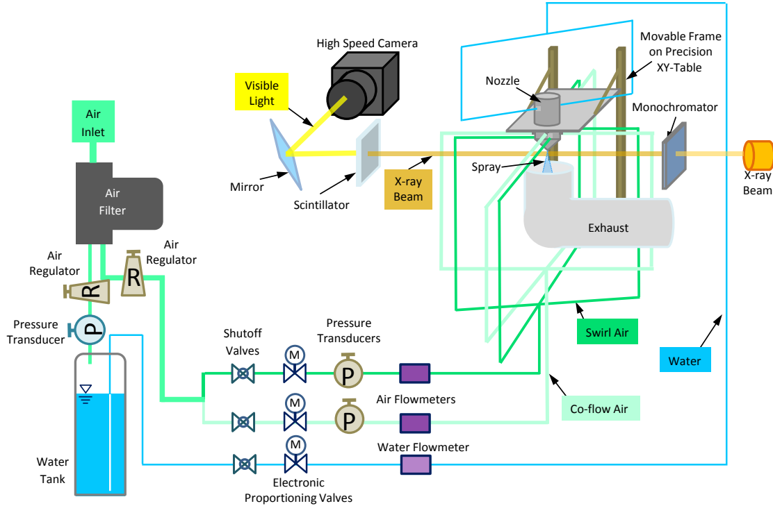
Figure 1 Schematic of the airblast atomizer setup for monochromatic beam imaging at the 7-BM beamline at the Advanced Photon Source.
