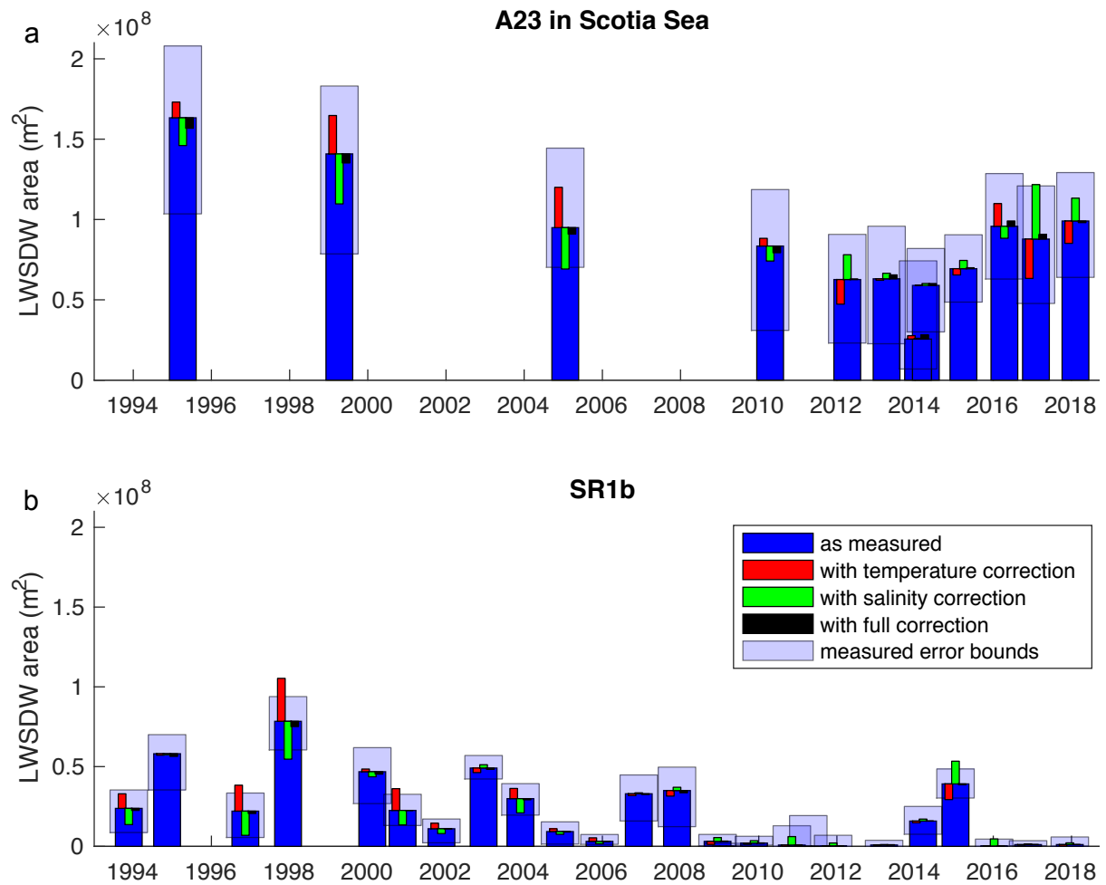
Figure 2. Area of LWSDW ( \gamma^n > 28.31 \text{ kg m}^{-3} ) from hydrographic sections. Panel a shows data from the A23 section in the Scotia Sea panel b is from the SR1b section. The blue bars are calculated from the measured properties; the red bars are compensated for the temperature anomalies on the \gamma^n = 28.31 \text{ kg m}^{-3} surface (as shown in Supplementary Information Figure 2 and discussed in more detail in Methods); the green bars are compensated for salinity anomalies; and the black bars are compensated for both temperature and salinity anomalies. The method used to compute the confidence limits (light blue bars) is described in the Methods section.
