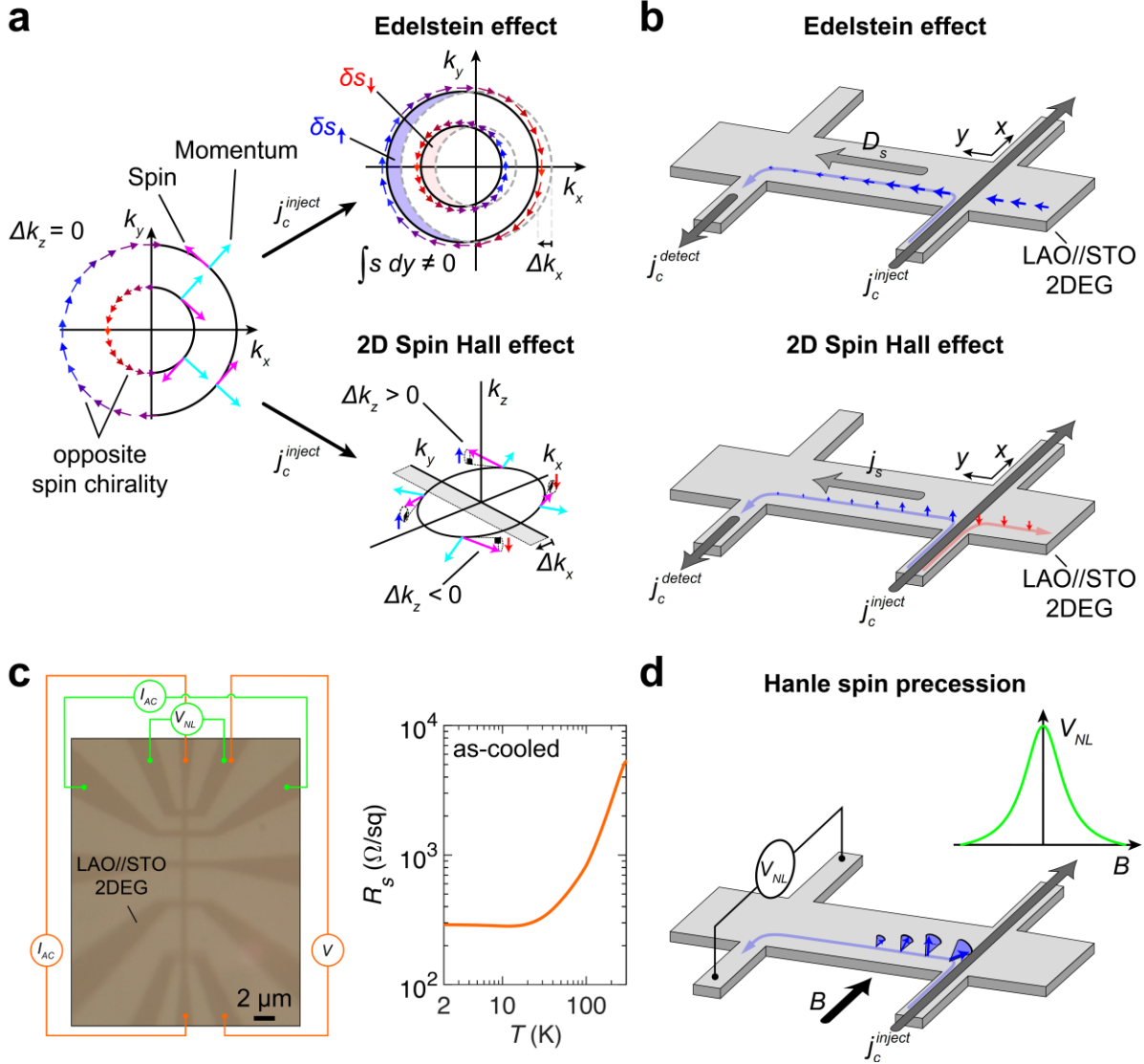
Figure 1. a , Because of the Rashba effect in \text{LaAlO}_3/\text{SrTiO}_3 (LAO//STO), the spin degeneracy is lifted, leading to concentric Fermi contours with opposite spin chirality where the spin is locked perpendicular to the momentum. Through the direct Edelstein effect an injected charge current ( j_c^{\text{inject}} ) along x will generate a transverse spin accumulation along y , \int s dy \neq 0 . Additionally, after displacing the Fermi contours by \Delta k_x , the spins will not be exactly perpendicular to k and will thus start to precess around to local Rashba field to eventually align along the new spin direction. While precessing, the spins acquire a finite component along +z for k_y > 0 and -z for k_y < 0 ; this is the two-dimensional (2D) spin Hall effect, which ultimately results in a net spin polarization along z . b , top panel, The spin accumulation generated by Edelstein effect will diffuse ( D_s ) along y in the Hall bar channel, before getting converted back into a detectable
