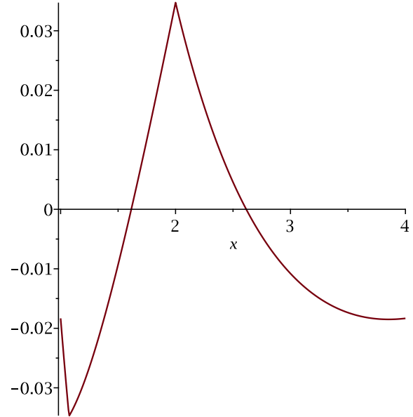
Fig. 10. Relative difference between Approximation (55) to \sqrt{x} with the constant 127 \cdot 2^{22} replaced by 532369100 and the actual \sqrt{x} in [1, 4] .
