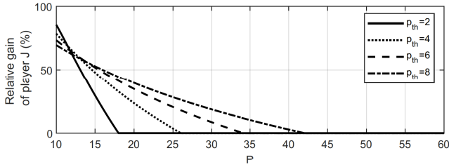
Fig. 4. Relative gain of player J , evaluated by function E , for different values of p_{th} for N = 10 , \sigma_J^2 = 1 and \Gamma = 4 .
