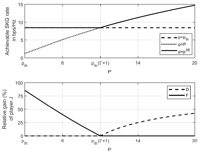
Fig. 2. UP: SE policy compared to always transmitting with either full power or with p_{th} . DOWN: Functions D and F vs P . In both sub-figures, p_{th} = 2 , \Gamma = 4 , N = 10 , \sigma^2 = \sigma_j^2 = 1 .
