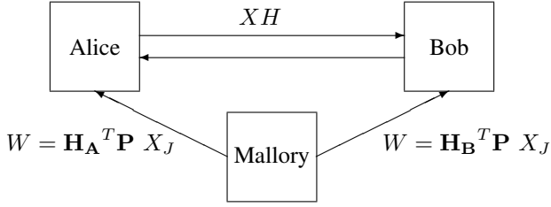
Fig. 1. Alice and Bob have single transmit and receive antennas and exchange pilot signals X over a Rayleigh fading channel with realization H . A MiM, Mallory, with multiple transmit antennas can inject a suitably pre-coded signal \mathbf{P}X_J , such that the received signal at both Alice and Bob coincide W = \mathbf{H}_A^T \mathbf{P} X_J = \mathbf{H}_B^T \mathbf{P} X_J .
