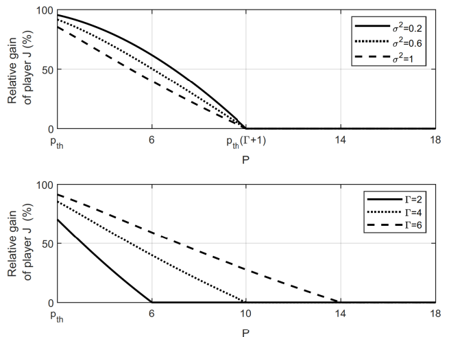
Fig. 3. Relative gain of player J , evaluated by function E , for strategic p_{th} and fixed p_{th} = 2 when N = 10 , \sigma_j^2 = 1 and UP: \Gamma = 4 , DOWN: \sigma^2 = 1 .
