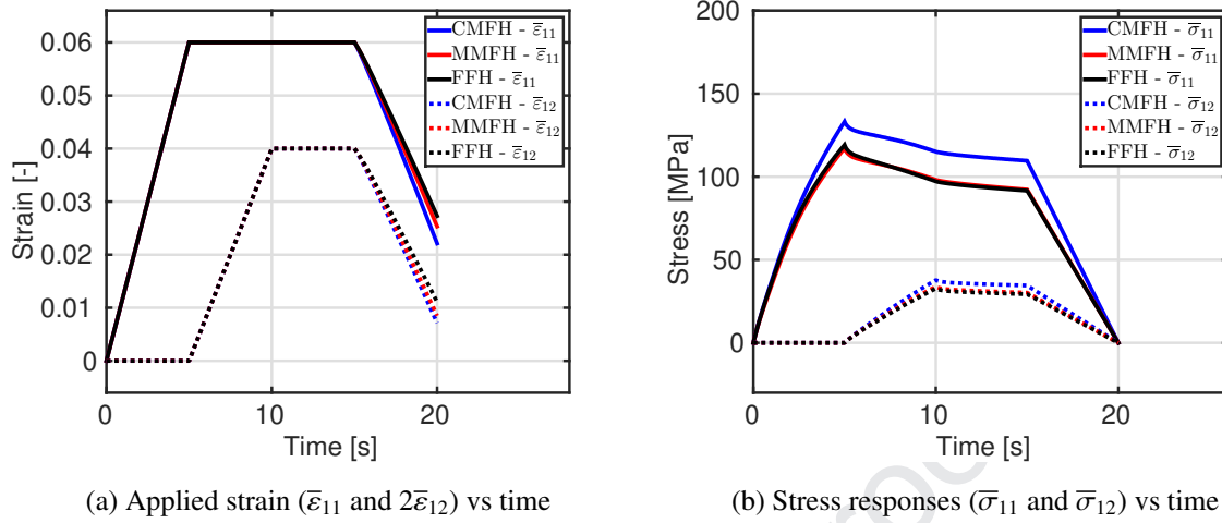
Figure 18: Complex non-proportional combined tension (1-1) and in-plane shear (1-2) virtual test on a VE-VP composite reinforced by 20% of long fibers, at the strain rates \dot{\epsilon}_{11} = 0.012 \text{ s}^{-1} and \dot{\epsilon}_{12} = 0.008 \text{ s}^{-1} . Comparison between the classical mean field homogenization model (CMFH), the modified mean field homogenization model (MMFH) and the reference full field homogenization model (FFH). It is recalled that the unloading stage is stress controlled.
