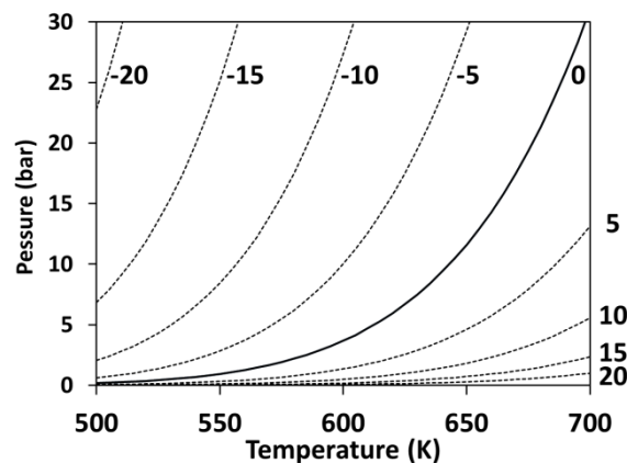
Figure 22. Calculated driving forces for hydrogen absorption/desorption in Mg as a function of temperature and pressure. Lines connect constant values, as indicated in \text{kJ mol}^{-1}_{\text{H}_2} . Thick continuous line corresponds to equilibrium conditions.
