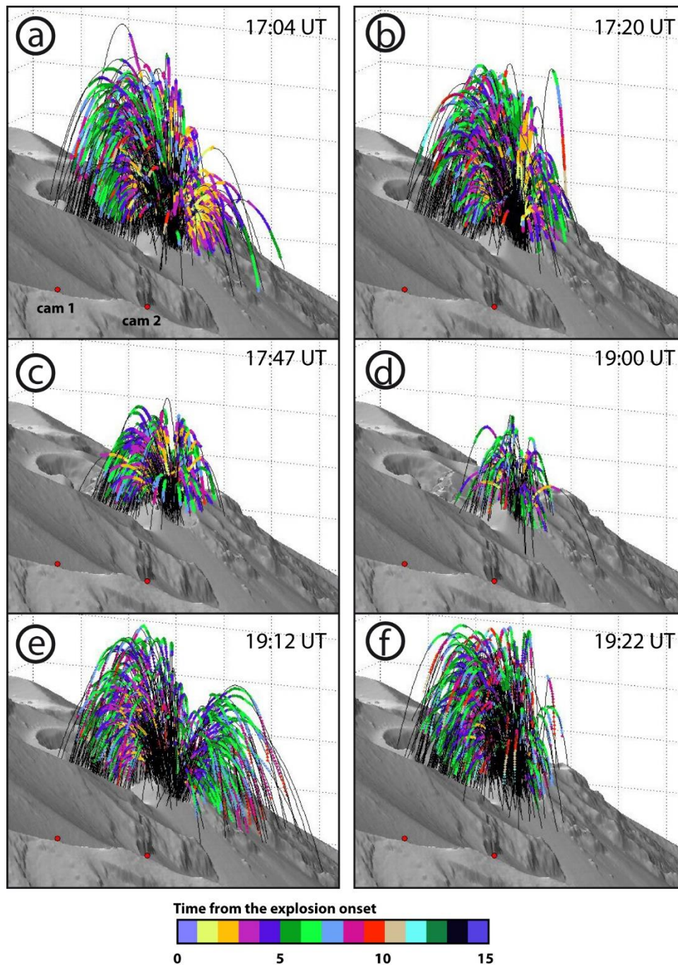
Fig. 5 3D reconstruction of the trajectories of 6 explosions on October 5, 2012. The colours indicate the time in seconds from the onset of the explosion. Black lines are parabolic fits of the trajectories
