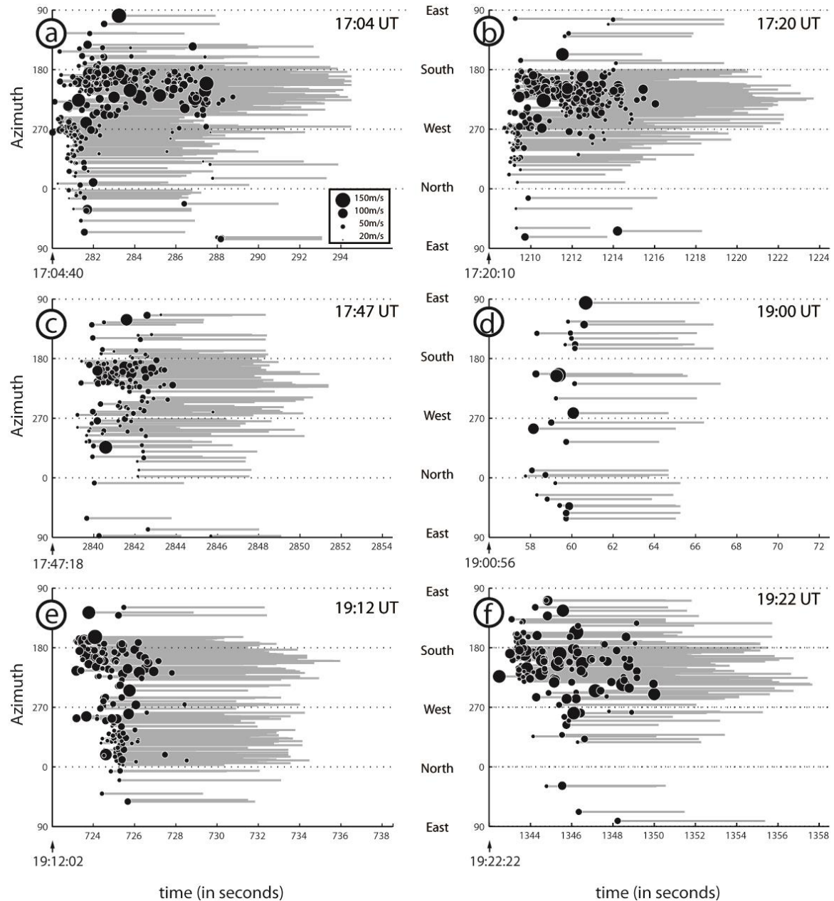
Fig. 7 Azimuth of the bomb ejection against time for the six eruptions studied on Oct. 5 2012. The horizontal axis is the time in seconds (a-c from 17:00 UT, and d-f from 19:00 UT). The black dots indicate the ejection time of each bomb and their size indicates the initial ejection velocity (see inset in 7a). The grey lines represent the time-period of the reconstructed trajectories (up to the point the bombs reach the ground, are masked by the topography or are too cooled to be detected)
