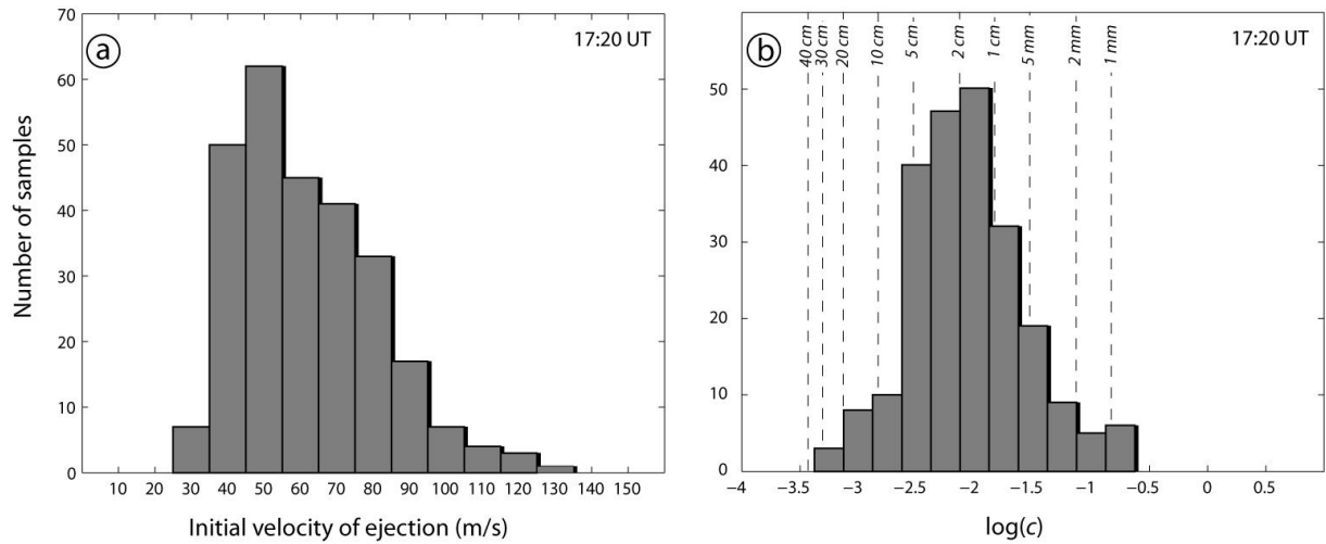
Fig. 9 (a) Histogram of calculated initial ejection velocities at the vent for the 230 bombs trajectories reconstructed during the 17:20 eruption using the model and its extrapolation. (b) Apparent drag coefficient c calculated using the model. The vertical lines indicate the radii corresponding to the values of c for Cd=0.7 and a bomb density of 1800 \text{ kg m}^{-3}
