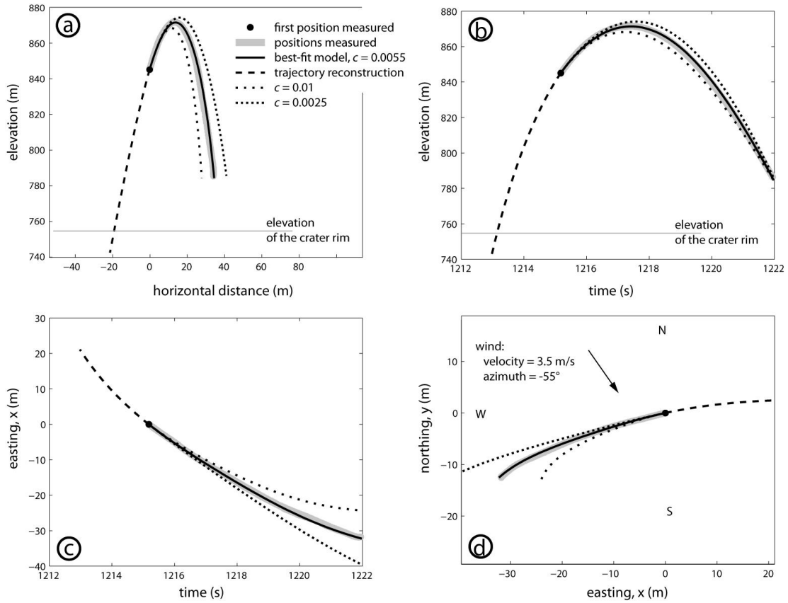
Fig. 8 Measurement of the 3D trajectory of bomb B (in grey; cf. Fig. 3) and simulations (in black) for 3 values of c (see Equation 8). The data are fitted in space (a, d) and time (b, c). The dashed line corresponds to the extrapolation of the bomb trajectory from its first detected position back to the vent using the best-fit values
