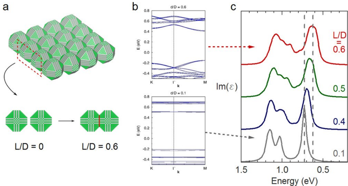
Figure 2. (a) Schematic representation of the model used in the tight binding calculations. The neck width L , the 2D projection of the epitaxial bond, is indicated by the red line. (b) The calculated electronic structures for superlattices with an L/D ratio of 0.6 (top) and 0.1 (bottom). For a low L/D ratio, the bands coincide with the energy levels of the individual NCs. At an increasing L/D ratio, dispersive bands start to form. (c) The dielectric function of the superlattice, calculated from the theoretical band structure. For L/D = 0.6 , the first excitonic transition red shifts by 99 meV and the fwhm increases by a factor 2.5 compared to the superlattice with L/D = 0.1 .
