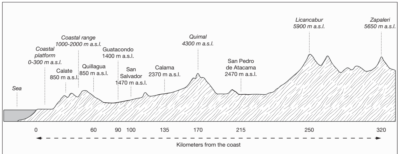
FIG. 2. — Altitudinal profile of the region with the position from the different localities mentioned in the article. Sites in italics: main geographical landmarks. Abbreviation: m a.s.l. , meters above sea level.
