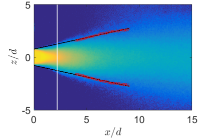
Figure 4. Visualization of the Spray Structure at Re_g = 4 \cdot 10^4 . Mean intensity field at the lowest liquid flow rate, phase \phi = \pi within the harmonic oscillation, showing the spray spreading rate from the 2\sigma intensity cutoff on a Gaussian fit to the radial evolution of the intensity, for different distances downstream of the nozzle.
