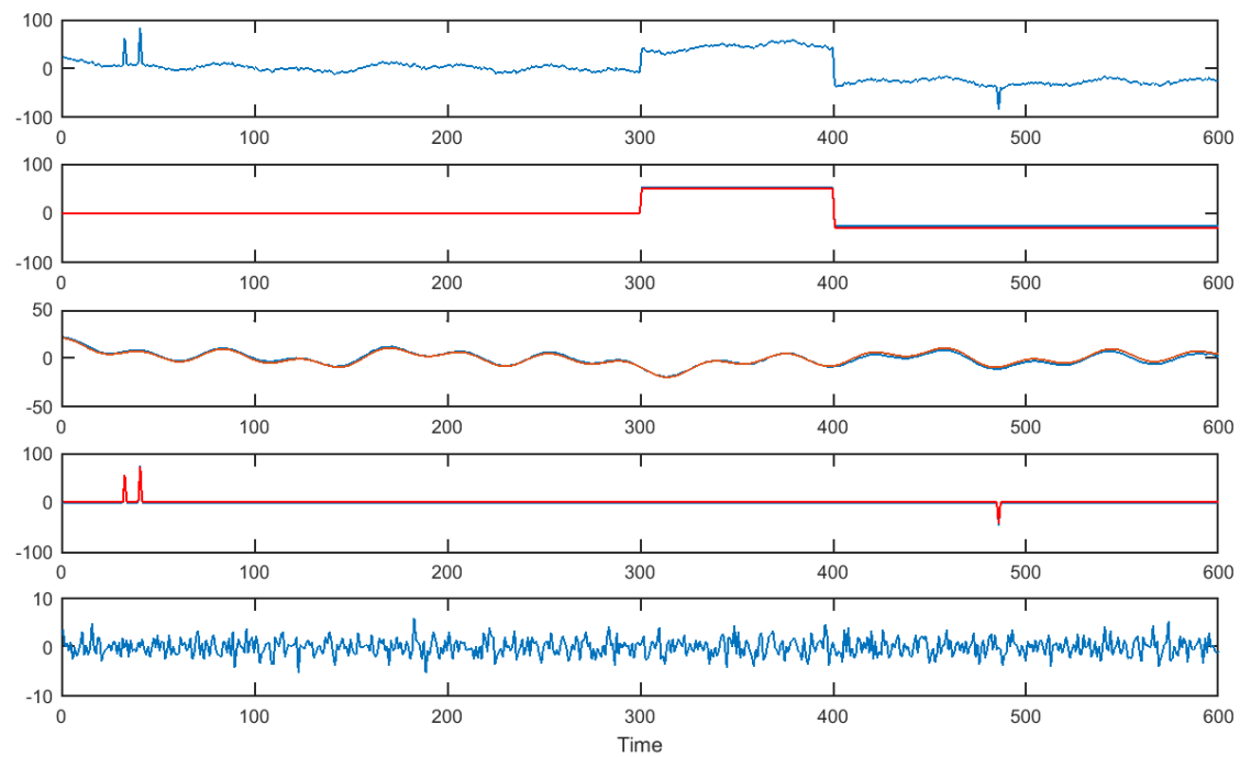
Figure 2. Decomposition of a signal with three outliers.
