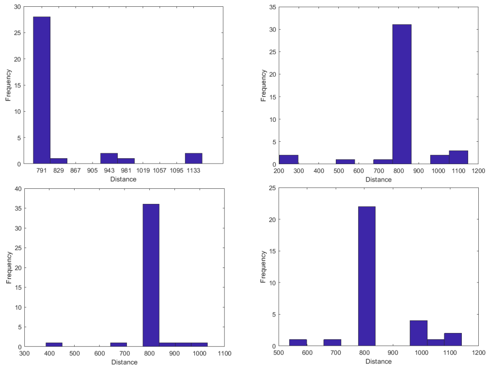
Figure 5. Histogram of distance measured for a minimum piecewise constant jump magnitude of 3\sigma (top left), 4\sigma (top right), 5\sigma (bottom left), and 6\sigma (bottom right).
