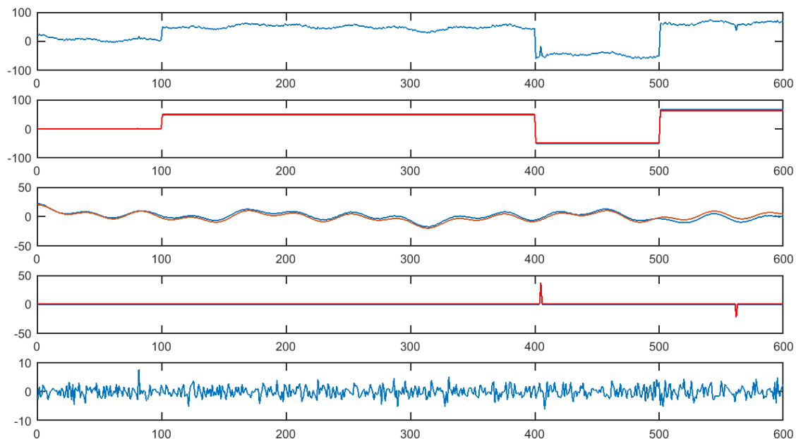
Figure 4. Decomposition of a signal with four piecewise constant jumps.
