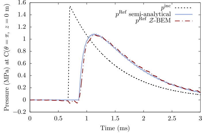
Figure 6: Scattering by a small cylinder ( a = 0.5 m, L = 5 m, see Fig. 5): comparison between the Z-BEM and semi-analytical solutions for the total field p^{\text{Ref}} on the z = 0 plane, at the standoff (a), orthogonal (b) and shadow (c) points. The incident field at those points is also shown.
