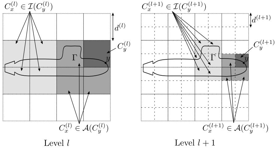
Figure 19: Illustration of the multi-level FMM in 2D. Both the interaction lists and the adjacent regions reduce in size as the level number increases.
