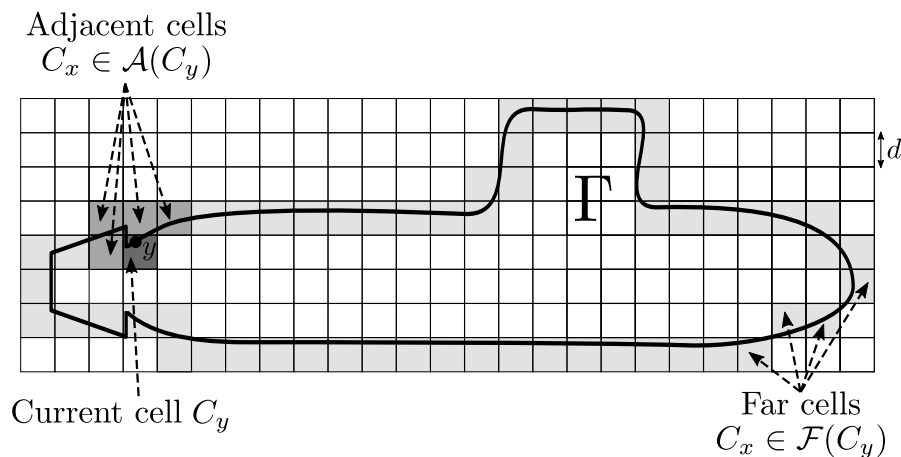
Figure 18: Two-dimensional grid embedding the boundary \Gamma . Definition of adjacent and far cells.
