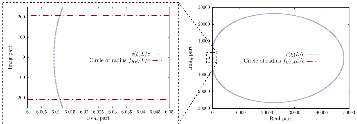
Figure 14: Scattering by a rigid motionless submarine: complex frequencies sL/c used by the Z -BEM. The frequencies for which a BEM problem is solved are concentrated near the origin.
