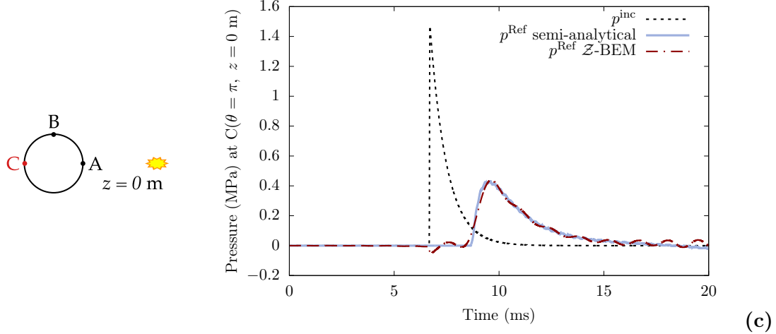
Figure 8: Scattering by a large cylinder ( a = 5 m, L = 50 m, see Fig. 5): comparison between the Z-BEM and semi-analytical solutions for the total field p^{\text{Ref}} on the z = 0 plane, at the standoff (a), orthogonal (b) and shadow (c) points. The incident field at those points is also shown.
