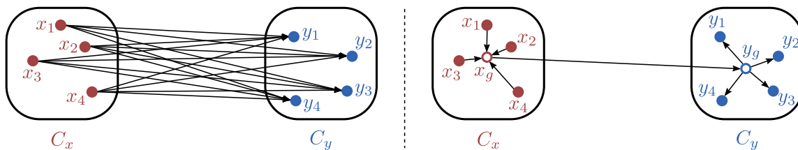
Figure 17: Illustration of the FMM concept, actions of the particles in a cell C_x (centre x_g ) on the particles in a cell C_y (centre y_g ). Left: without FMM, right: with FMM.
