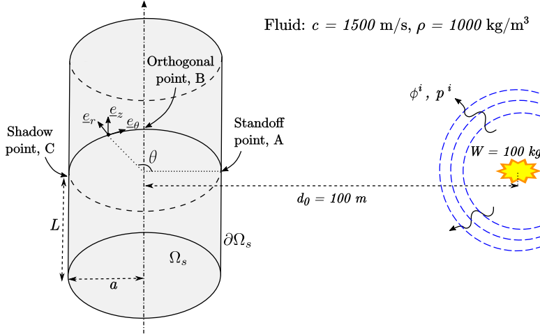
Figure 5: Infinite cylinder facing an underwater explosion.
