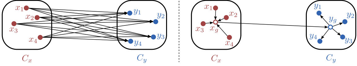
Figure 17: Illustration of the FMM concept, actions of the particles in a cell C_x (centre x_g ) on the particles in a cell C_y (centre y_g ). Left: without FMM, right: with FMM.
