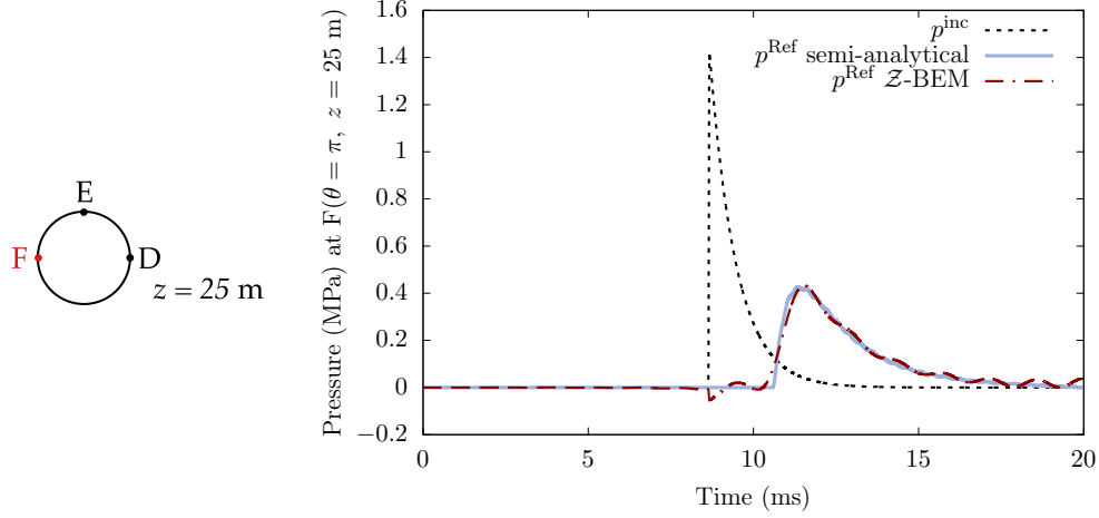
Figure 9: Scattering by a large cylinder ( a = 5 m, L = 50 m, see Fig. 5): comparison between the Z-BEM and semi-analytical solutions for the total field p^{\text{Ref}} on the z = 25 m plane, at the standoff (a), orthogonal (b) and shadow (c) points. The incident field at those points is also shown.
