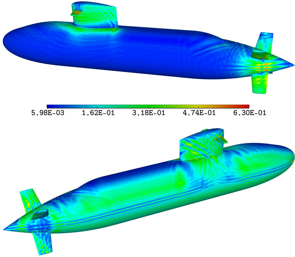
Figure 13: Scattering by a rigid motionless submarine: relative oscillation \Delta_{HFA}(\mathbf{y}) of \mathbf{y} \mapsto \Delta_{HFA}(\mathbf{y}) plotted as a function of \mathbf{y} \in \Gamma . BEM solutions for N_B = 56 complex frequencies were computed.
