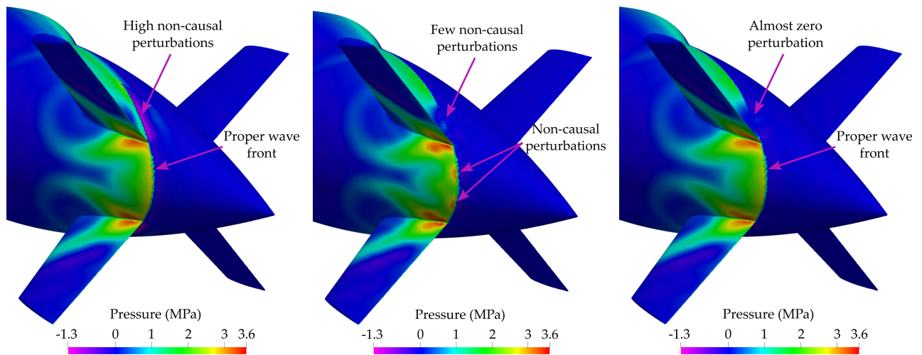
Figure 16: Scattering by a rigid motionless submarine: total pressure field on the surface, 5.4 milliseconds after the incident wave first hits the submarine. Close-up on the back part for three variants of the HFA, based on the Kirchhoff approximation (left), \mathcal{R}(\mathbf{y}, s_{\text{HFA}}) (middle) or an average of \mathcal{R}(\mathbf{y}, \cdot) (right).
