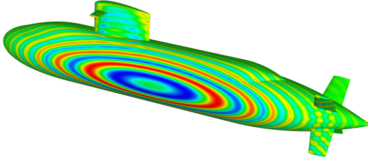
Figure 11: Scattering by a rigid motionless submarine: \mathcal{Z} -transform of the total pressure P^{\text{Ref}}(s) on the submarine surface, with sL/c \approx 6.01 + 166i .
