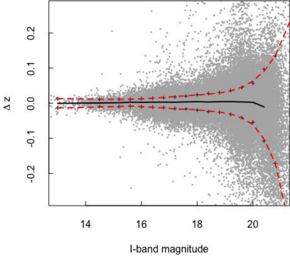
Fig. 2. Relation (Photometric redshifts–Spectroscopic redshifts)/(1 + Spectroscopic redshifts) ( \Delta z ) vs. i -band cModel magnitude for a sample of galaxies with both spectroscopic and photometric redshifts in SDSS DR14 (gray dots). The black pluses and black solid line show the dispersion and peak of the Gaussian fitted in each i -band magnitude bin, respectively. There are in total 17 bins. The red dashed lines indicate the model fitted to the dispersions.
