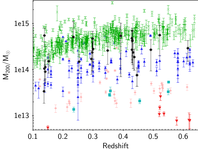
Fig. 1. Cluster M_{200} –redshift plane for CODEX-SPIDERS (green cross), AEGIS (cyan filled square), COSMOS (pink diamond), CDFS (point down red triangle), XMM-CFHTLS (point-up blue triangle), and XMM-XXL (black filled circle) surveys used in this work.
