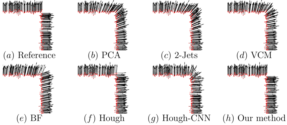
Figure 5: 2D projection of the normal estimations on the intersection of two planes.
