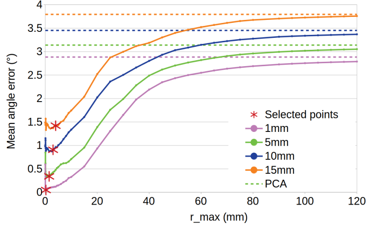
Figure B.20: Mean angle error evaluated on the intersection of two planes ( 1 \times 0.5 m) randomly sampled by 15 000 points. The value of r_{max} is increased (please refer to text for variables definition). The neighborhood is defined by 300 points. The evaluation is performed for 4 Gaussian noise levels (noise level expressed as the standard deviation in mm). The errors resulting from PCA normal estimations are represented with dashed lines.
