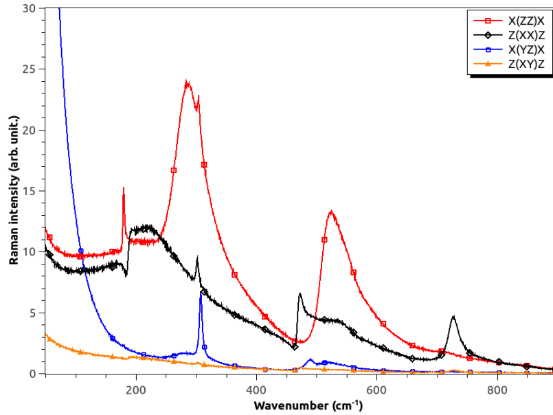
Figure 1. Polarized Raman spectra recorded at room temperature on a single-domain BaTiO 3 crystal.
