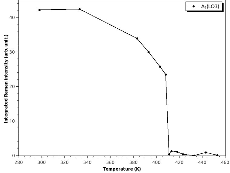
Figure 3. Temperature dependence of the integrated intensity J of the A_1(\text{LO}3) peak in single-domain \text{BaTiO}_3 crystal. J is calculated by integration after subtraction of a linear baseline. Above T_c the non-zero value of the intensity can be related to pre-transitional features extensively reported in literature [26].
