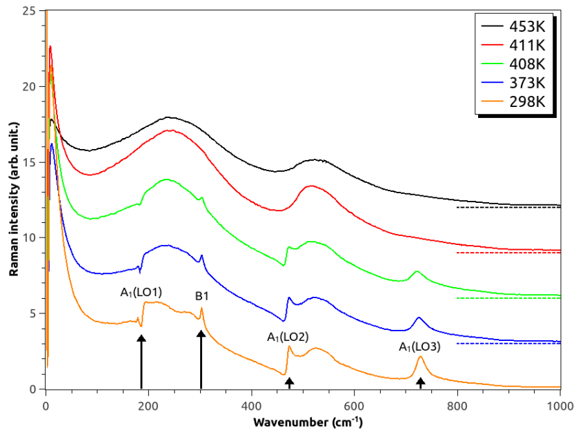
Figure 2. Z(XX)Z Raman spectrum recorded at different temperatures on a single domain BaTiO 3 crystal. The arrows indicate the position of the first-order lines A 1 (LO) and B 1 . The dashed line corresponds to zero intensity line for each temperature.
