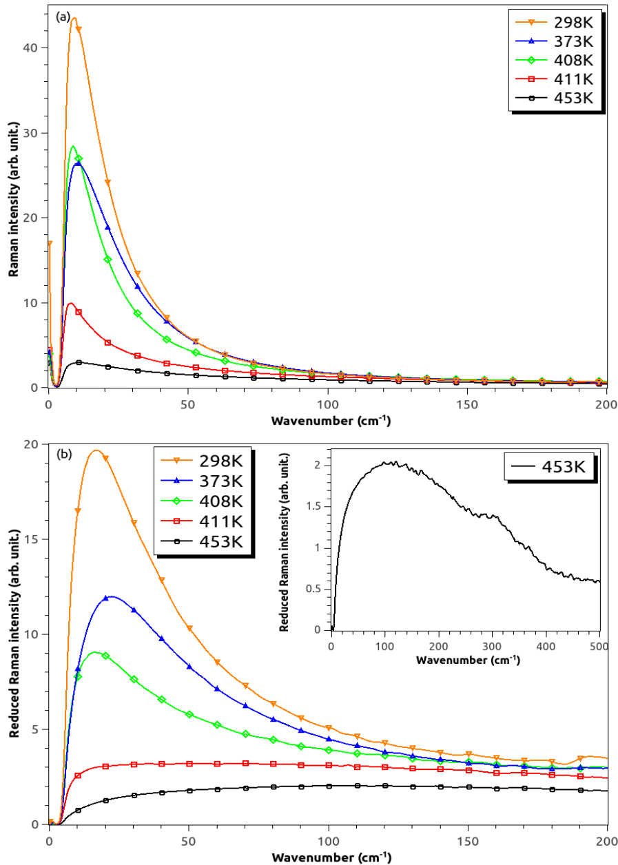
Figure 5. Low- frequency Z(XY)\bar{Z} Raman spectrum recorded at different temperatures on single \text{BaTiO}_3 crystal: (a) raw data, (b) corrected data according to eq 2. Inset: spectrum measured in the
