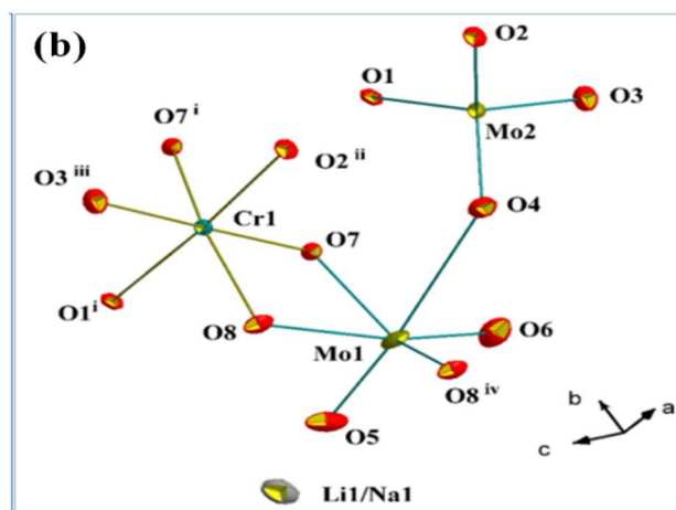
Fig.1: The structural unit of \beta -Li 0.87 Na 0.13 Cr(MoO 4 ) 2 ,
