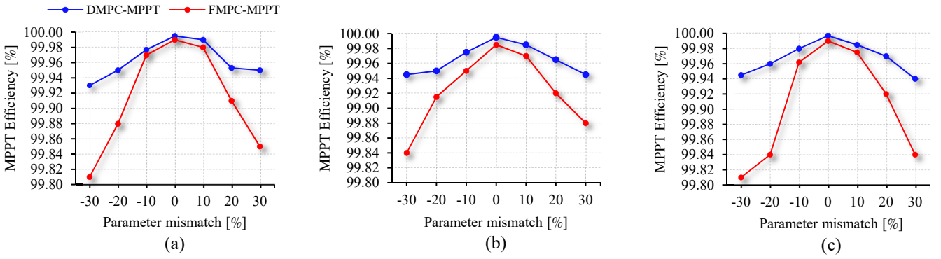
Fig. 14. Simulation results of FMPC-MPPT and DMPC-MPPT efficiencies under STC, and in case of model parameter mismatch using: (a) Boost converter “ L and C_2 ”, (b) Z-source inverter “ C_1 and L_1 ”, and (c) Flyback converter “ C and L_m ”.
