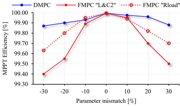
Fig. 17. Experimental results of FMPC-MPPT and DMPC-MPPT efficiencies under STC in case of model parameter mismatch “ L and C_2 ”. The red dash line represents FMPC efficiencies with load value misestimated “ R_{load} ”.
