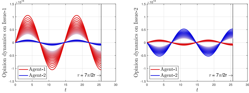
Figure 1: Oscillating opinion trajectories for \tau \in [c_3 - 10^{-9}, c_3) with increasing magnitude as \tau \rightarrow c_3 = 7\pi/2r
