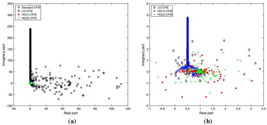
Fig. 1 Unit sphere. Distribution of the eigenvalues of the standard and three P-CFIEs ( \eta = 1, \kappa_s = \omega = 50 and n_{\lambda_s} = 12 ). a Complete distribution and b Closer view on the clustering
