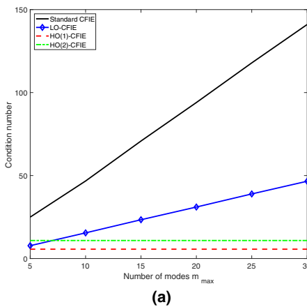
Fig. 3 Unit disk. Study of the condition number of the P-CFIEs. a Condition number with respect to the maximal number of modes m_{\max} ( \kappa_s = 4\pi ). b Condition number with respect to the frequency ( n_{\lambda_s} = 12 )
