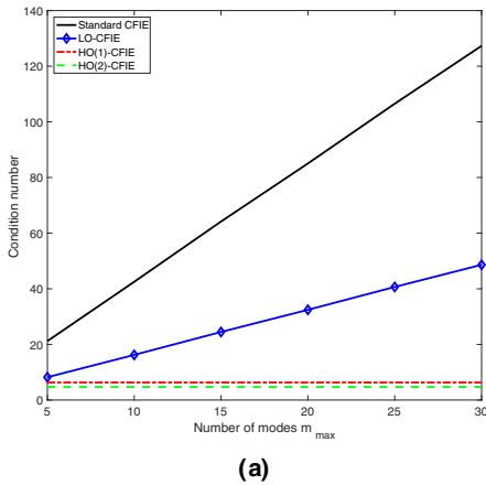
Fig. 2 Unit sphere. Study of the condition number of the three P-CFIEs. a Condition number with respect to the maximal number of modes m_{\max} ( \kappa_s = 4\pi ). b Condition number with respect to the frequency \omega ( n_{\lambda_s} = 12 )
