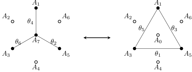
Figure 16: Star-triangle transformation on G (black vertices)
