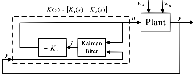
Fig. 4. General scheme of LQG controller.
