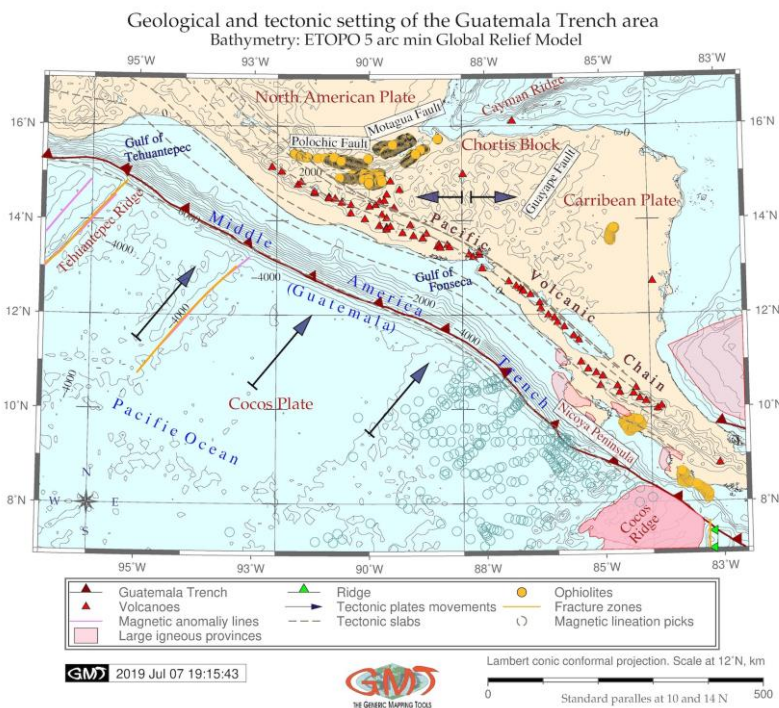
Figure 2. Geological settings of the Guatemala Trench
