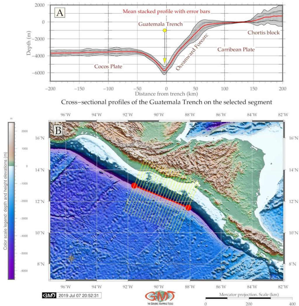
Figure 10. Cross-section profiles on the selected segment of the Guatemala Trench
