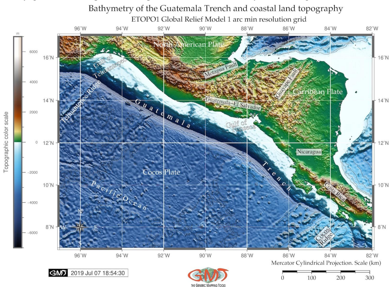
Figure 1. Bathymetry of the Guatemala Trench. Cartographic base data: ETOPO1.
