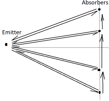
Figure 11: In case of race, an absorber only receive a half photon or a part of photon, in this case the energy is allowed to be returned through the time-reversal mutual energy flow. In this way, the energy on the detector screen can flow from one absorber to another. Once an absorber received an energy of whole photon, it will locked this energy and does not allow this energy to return. The energy is sent form the emitter to the absorber in this way.
