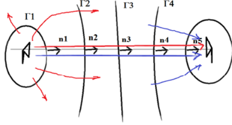
Figure 10: Mutual energy flow is consist of the retarded wave and the advanced wave. Retarded wave is shown as red curve, the advanced wave is shown as blue curve. Mutual energy flow are equal at any surface between the emitter and the absorber.
