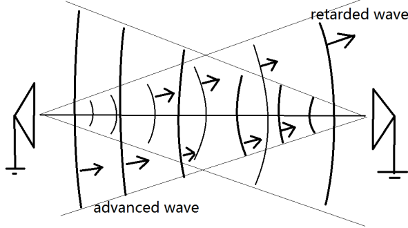
Figure 6: This figure shows the two waves are synchronized, one is a 3-D retarded wave and another one is a 3-D advanced wave
