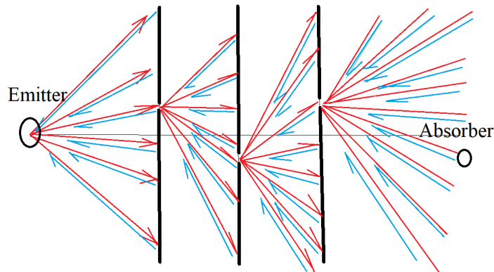
Figure 12: There is a emitter and absorber. Between the emitter and the absorber there are a few partition boards. On the partition boards there is a hole for each board to allow light to go through. This figure shows the retarded wave collapse on each hole. Red line is the retarded wave. Blue line is the process of the collapsed wave. The retarded wave collapse on holes of each partition board. In the end the wave collapses at the absorber. This is unbelievable.
