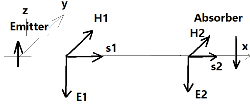
Figure 2: photon model, in this model the field \zeta_1 = [\mathbf{E}_1, \mathbf{H}_1, \mathbf{J}_1], \zeta_2 = [\mathbf{E}_2, \mathbf{H}_2, \mathbf{J}_2] all satisfy SCMEQ.
