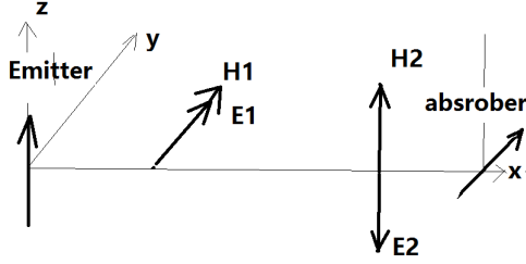
Figure 4: In this photon model, the fields \zeta_1 = [\mathbf{E}_1, \mathbf{H}_1, \mathbf{J}_1], \zeta_2 = [\mathbf{E}_2, \mathbf{H}_2, \mathbf{J}_2] do not satisfy the SCMEQ. However, they still satisfy the mutual energy principle.
