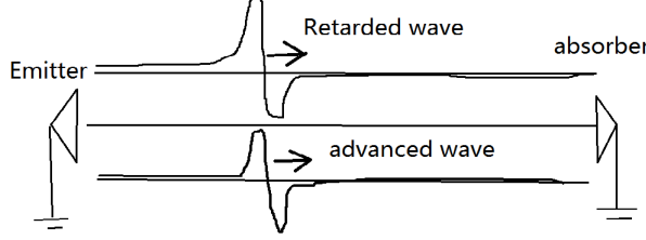
Figure 5: This figure shows the two waves are synchronized, one is a 1-D retarded wave and another one is a 1-D advanced wave
