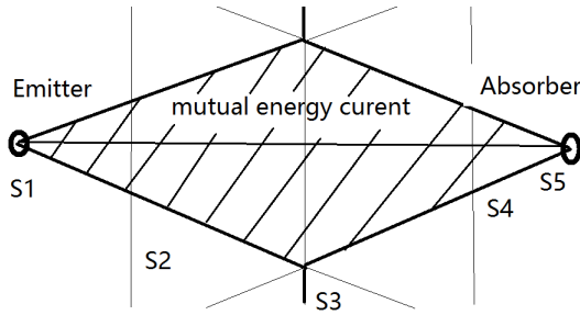
Figure 3: The mutual energy flow only exists at the overlap place of the two solutions of the SCMEQ. The field of the emitter is retarded wave. The field of the absorber is advanced wave.
