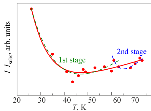
Fig. 7. (Color online) Temperature dependence of the diffraction intensity excess averaged over the 1st broad peak as shown in Fig. 6 relative to a signal from a carbon substrate. This access exhibits the exponential decay with T and a noticeable two-stage character of Ar desorption in a wide temperature range up to T values more than twice higher as compared with the sublimation point of polycrystalline argon in vacuum conditions of the used setup.
