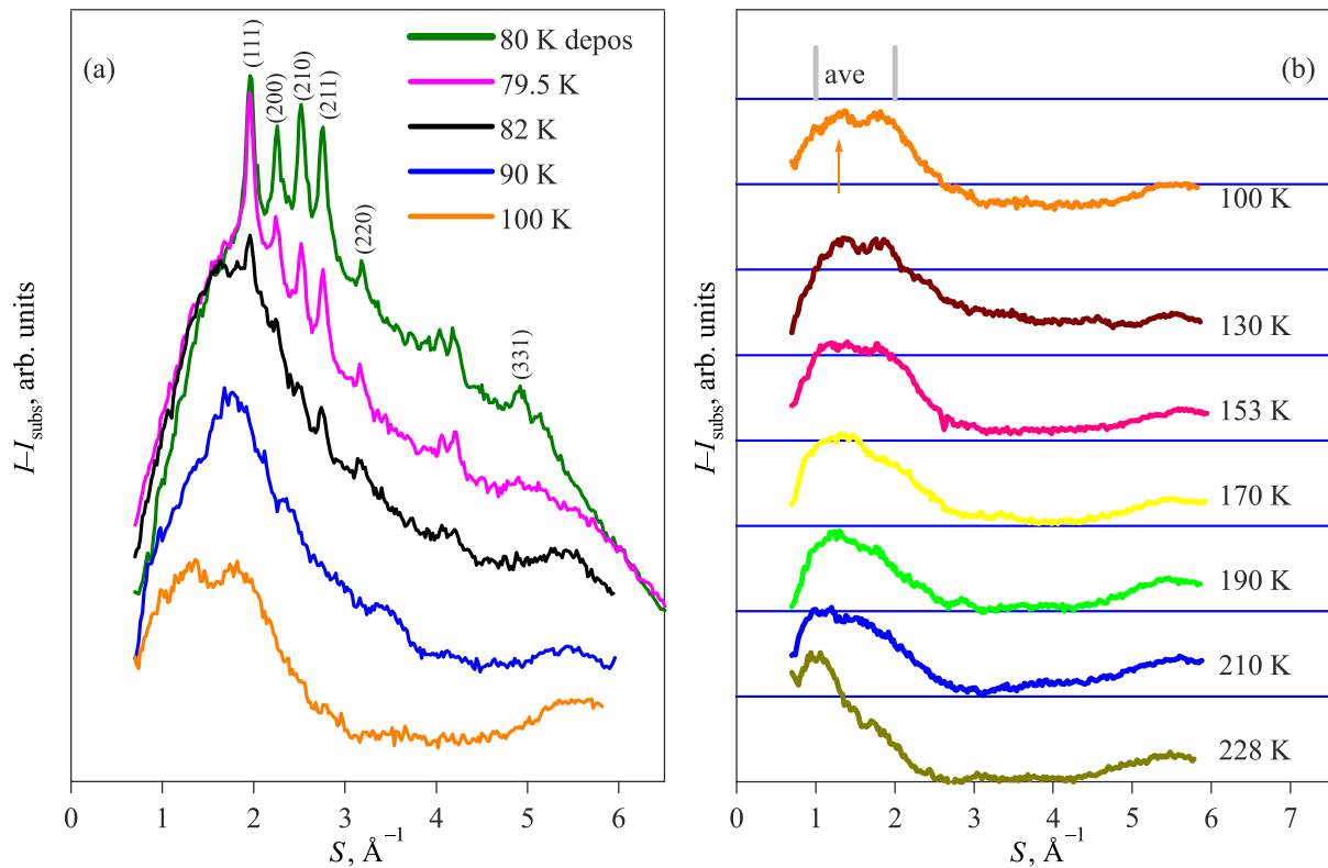
Fig. 9. (Color online) The excess I-I_{\text{subst}} of experimental diffraction intensities from composites formed by carbon dioxide absorbed in carbon honeycomb matrices during deposition closely to T_{\text{subl}} of \text{CO}_2 in vacuum relative to the intensities from a carbon substrate (a). On the right (b) the differences I-I_{\text{subst}} are shown at elevated temperatures and shifted along vertical to make details visible. A wide but well defined peak is attributed to molecules with short range order captured in the carbon honeycomb matrices and is still visible up to \sim 230 K (maximal T attained in this experiment) that is about three times higher as compared with T_{\text{subl}} \sim 86 K for \text{CO}_2 under typical vacuum conditions in the used setup [6].
