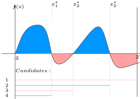
Figure 2: Example of computation of \int_{\bar{x}}^{[x]} f(x)dx for \mathcal{X}_2^* = \{x_1^*, x_2^*, x_3^*\} .
