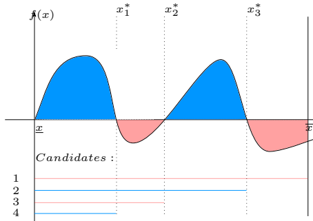
Figure 2: Example of computation of \int_{\underline{x}}^{[x]} f(x)dx for \mathcal{X}_2^* = \{x_1^*, x_2^*, x_3^*\} .
