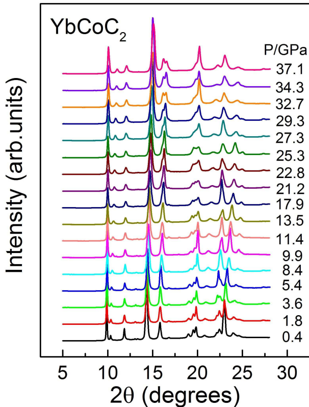
Fig. S 2. X-ray diffraction patterns of YbCoC 2 at different pressures.
