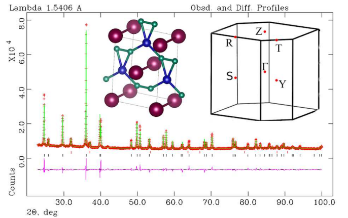
Fig. S 1. XRD pattern for \text{YbCoC}_2 at room temperature and P = 0 GPa (the obtained lattice parameters are listed in Table I). The experimental points (red marks), the calculated profiles (green line) and their difference (purple line) are shown. The bars in the lower part of the graph represent the calculated Bragg reflections that correspond to the \text{YbO} impurity phase (upper row, red color) and \text{YbCoC}_2 (lower row, blue color). Inset: The unit cell (generated using the VESTA software [5]), with the red, blue and green balls corresponding to Yb, Co and C ions (left) and the first Brillouin zone (right) of the Amm2 structure of \text{YbCoC}_2 .
