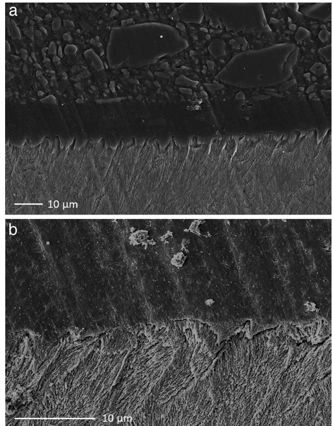
Figure 7. SEM of the interface enamel/infiltrant/adhesive (bracket not visible) for the ERI+1 group at 1000 \times (a) and 3000 \times (b) magnification.
