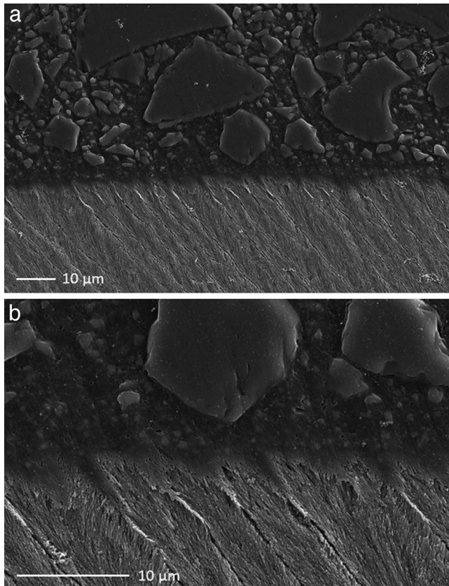
Figure 2. SEM of the interface between eroded enamel and adhesive (bracket not visible) at 1000 \times (a) and 3000 \times (b) magnification.
