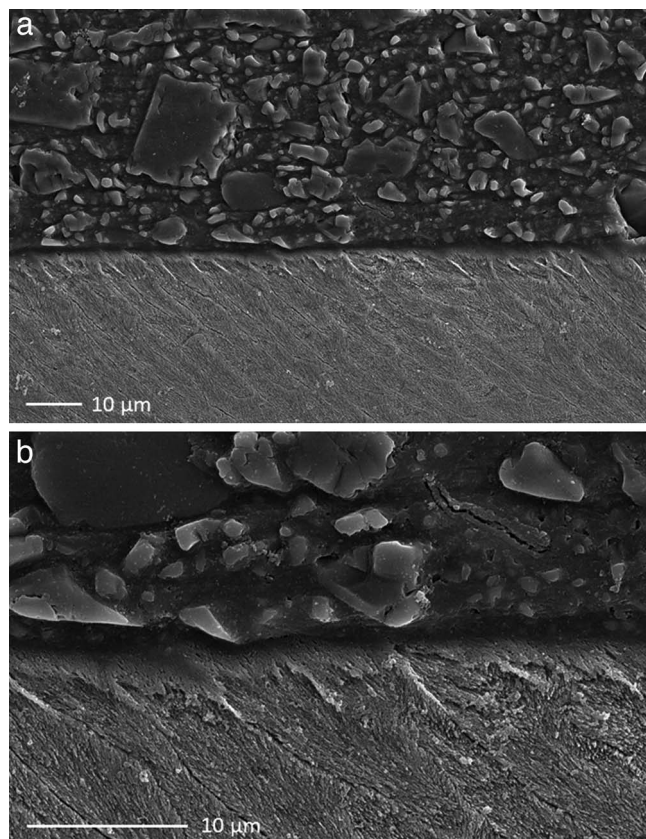
Figure 4. SEM of the interface enamel/infiltrant/adhesive (bracket not visible) for the IRI group at 1000 \times (a) and 3000 \times (b) magnification.
