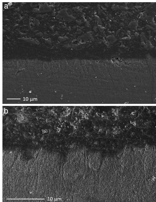
Figure 1. SEM of the interface between sound enamel and adhesive (bracket not visible) at 1000× (a) and 3000× (b) magnification.
