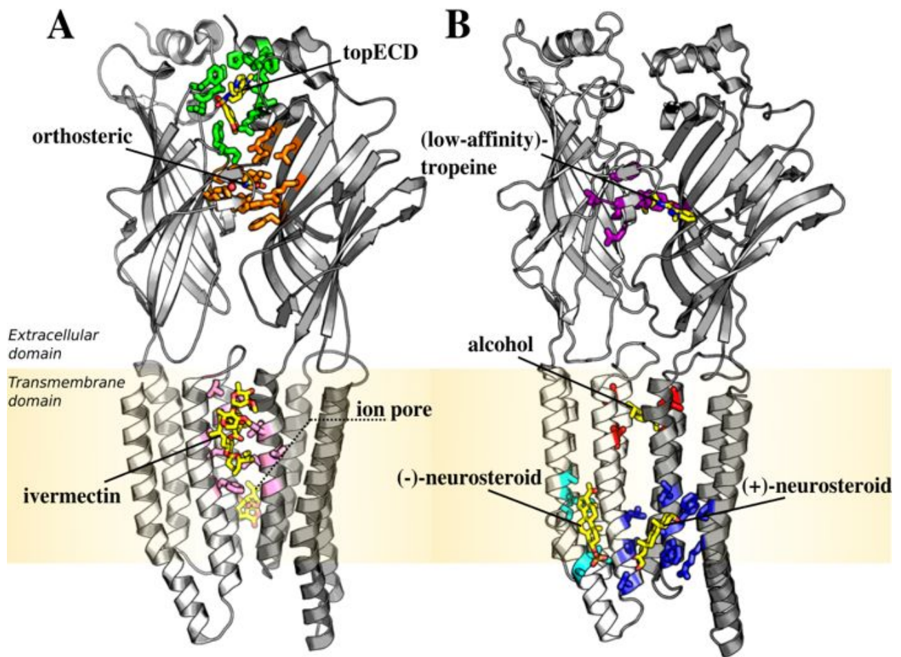
Figure 2. Topographical location of the actual/putative regulatory sites at GlyR by structural biology. (A) Regulatory sites illuminated by high-resolution structures of GlyR. From top to bottom: (1) the allosteric inter-subunit extracellular site (topECD) that accommodates the positive allosteric modulator AM-3607 is shown in green; (2) the orthosteric site that binds the endogenous neurotransmitter glycine is in orange; (3) the allosteric inter-subunit site in the transmembrane domain that binds the positive allosteric modulator ivermectin (ivermectin site) is in pink; (4) the allosteric site for negative modulation by picrotoxin (ion pore site) is in the background. Coordinates for glycine, the allosteric modulators AM-3607 and ivermectin were extracted from the X-ray structure of GlyR- \alpha 3 (PDB: 5VDH) (Huang, Chen and Shaffer, 2017). Coordinates for picrotoxin were extracted from the X-ray structure of GABA A - \alpha 1\beta 3\gamma 2 (PDB: 6HUG) (Masiulis et al., 2019); they are consistent with the most-recent cryo-EM results in GlyR- \alpha 1 (Kumar et al., 2019). (B) Putative regulatory sites illuminated by high-resolution structures of homologous pLGICs with concordant evidence at GlyR. From top to bottom: (1) the extracellular site for the low-affinity tropeine-binding site is shown in purple with granisetron bound; (2) the inter-subunit transmembrane site for alcohol binding is in red with propofol bound; (3) the allosteric intra-subunit for inhibition by neurosteroids or (-)-neurosteroid site is shown in cyan with pregnenolone sulfate bound; (4) the allosteric inter-subunit binding site for potentiation by neurosteroids or (+)-neurosteroid site is shown in dark blue with tetrahydrodeoxycorticosterone (THDOC) bound. Coordinates for THDOC and pregnenolone sulfate were extracted from the X-ray structures of GLIC-GABA A - \alpha 1 chimera (PDB: 5OSB) and (PDB: 5OSC), respectively, (Lavery et al., 2017), after structural alignment to GlyR- \alpha 3 in PyMOL (Schrödinger, 2015). Coordinates for granisetron were extracted from the high-resolution structure of 5-HT 3A receptor (PDB: 6NP0) (Basak et al., 2019). Coordinates for propofol were extracted from the high-resolution structure of GLIC F238A/N239A (PDB: 5MVM) (Fourati et al., 2018). In all cases, residues that are known to be involved in binding of allosteric modulators at GlyR are color-coded.
