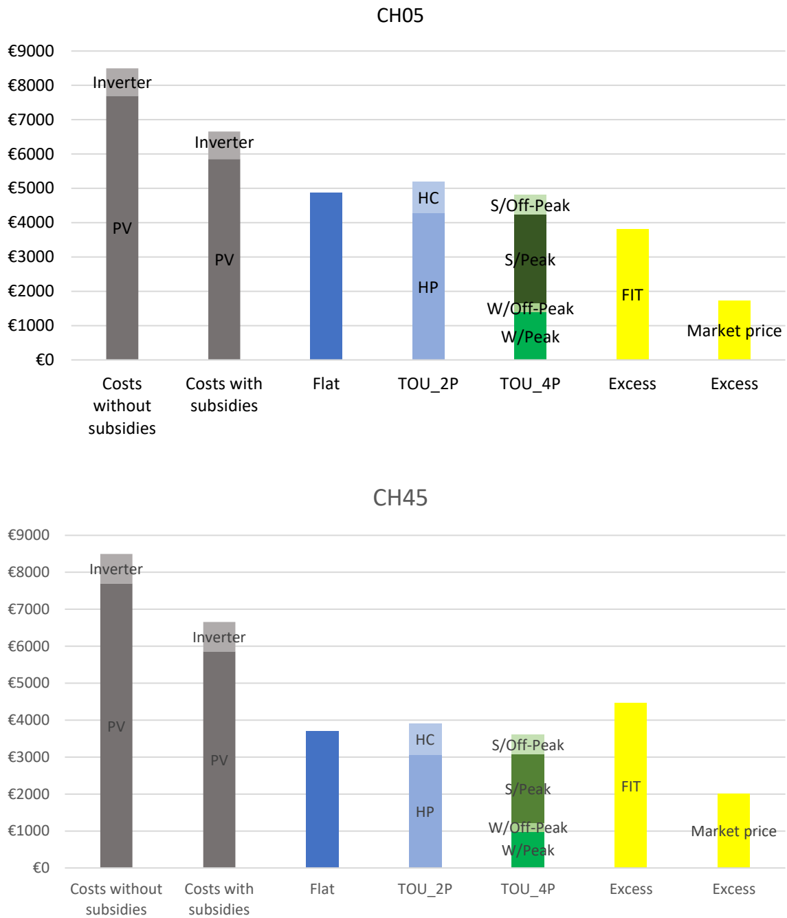
Figure 10: Breakdown of the costs and incomes from a 3 kW PV (W: Winter; S: Summer)
