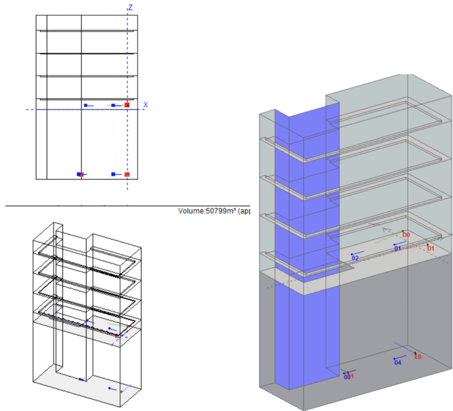
Figure 3: GA model of the Atrium V2, extended to include the sub space Galleria, from which the intrusive noise was coming.
