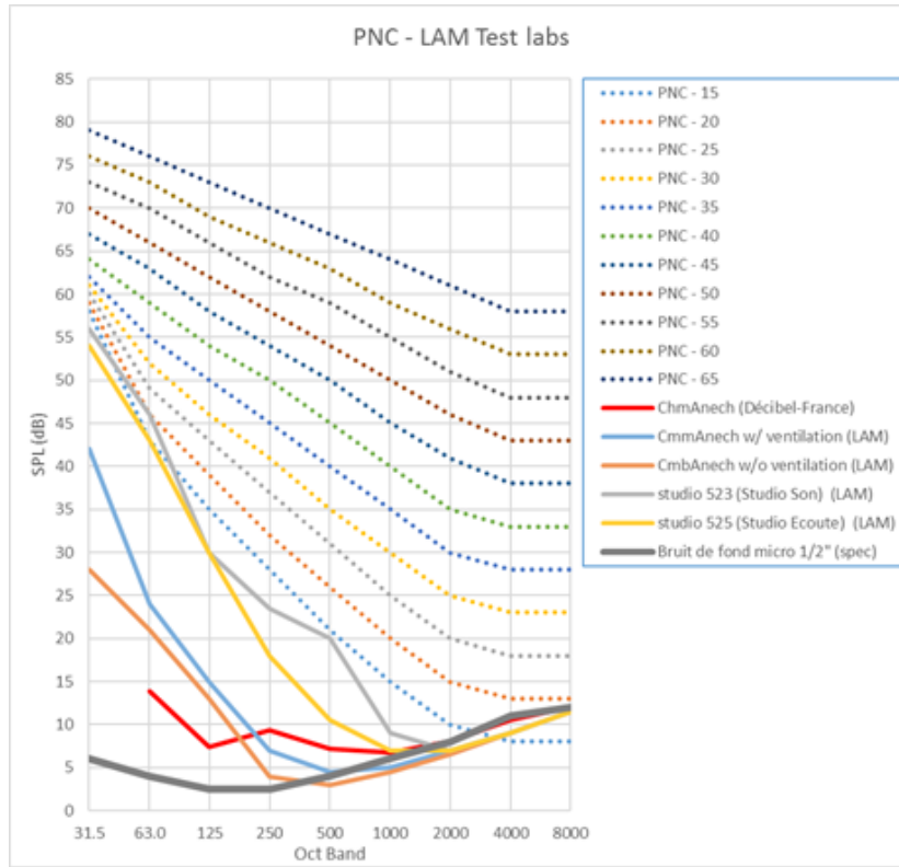
Figure 7: PNC curves representing the SPL level as a function of frequency, in addition to noise level in the different spaces of the University. Of interest are Studio 523 (Gray) and Anechoic chamber (Orange).
