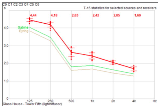
Figure 2: Reverberation times in the Atrium for the various S-R pairs.
