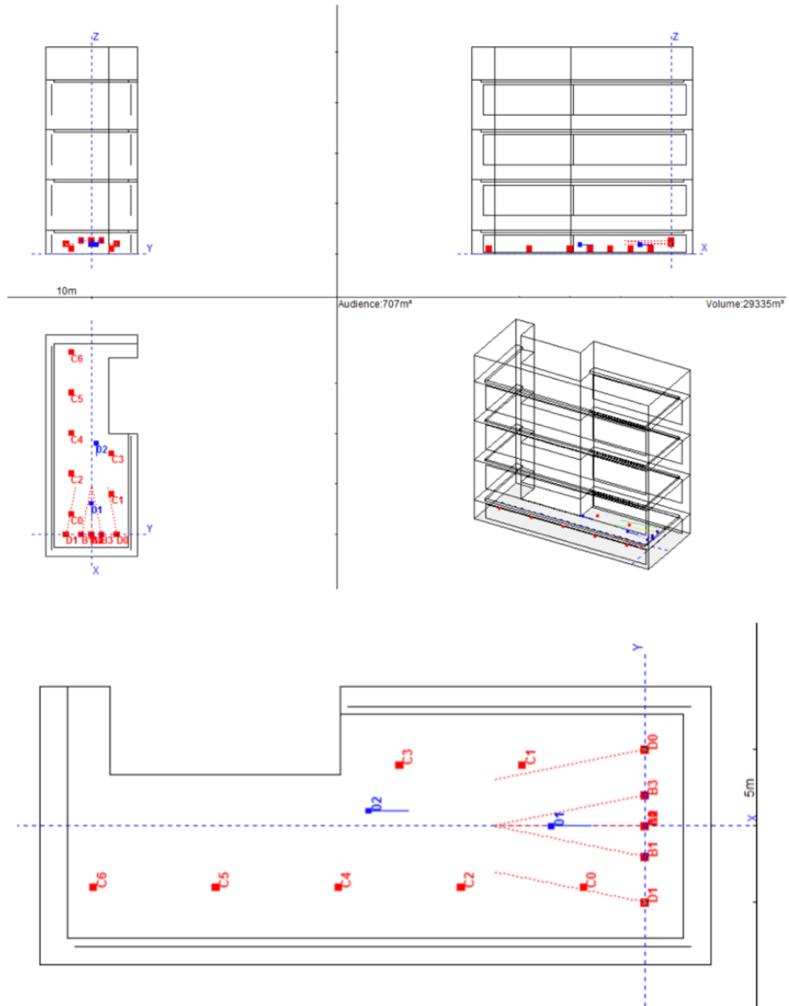
Figure 1: GA model of the Atrium, showing sources (in red) and receivers (in blue) positions.
