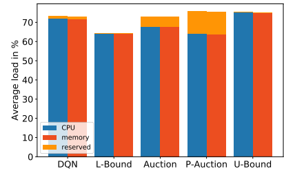
Fig. 13. Average load for 20 robots
