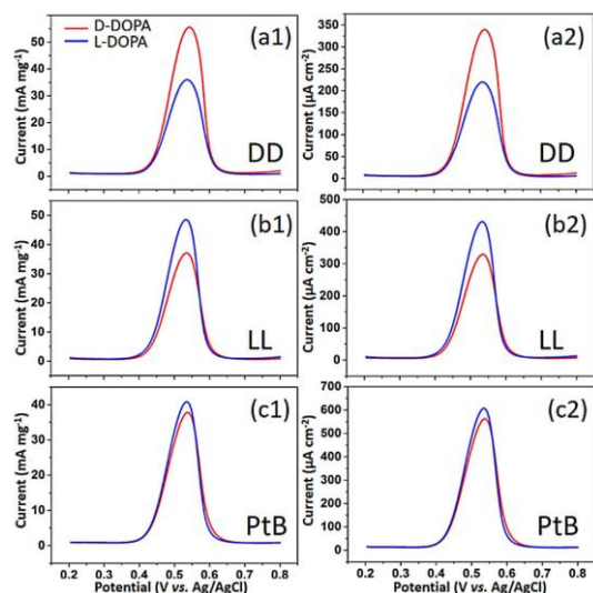
Figure 6. Chiral recognition of DOPA enantiomers recorded by differential pulse voltammetry (DPV) with (a) Pd@Pt particles that were synthesized in the presence of D-DOPA and D-AA (ascorbic acid), (b) Pd@Pt particles that were synthesized in the presence of L-DOPA and L-AA, and (c) Pt black (PtB) recorded in 4 mM DOPA in 50 mM HCl from 0.2 V to 0.8 V. Reproduced with permission from Ref[24]. Copyright (2017) Wiley-VCH Verlag GmbH & Co. KGaA, Weinheim.
