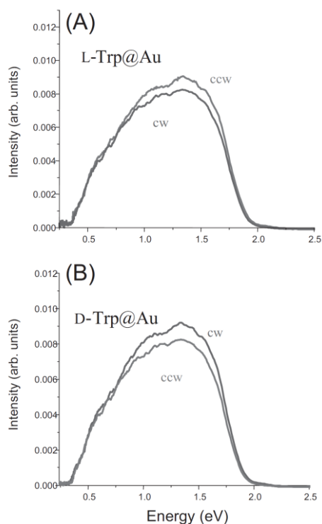
Figure 2. Illustration of the electron energy distribution profiles of photoelectrons ejected by ccw-CPL and cw-CPL on gold embedded with tryptophan enantiomers: A) L-Trp@Au and B) D-Trp@Au. Reproduced with permission from Ref[18]. Copyright (2007) WILEY-VCH Verlag GmbH & Co. KGaA, Weinheim.
