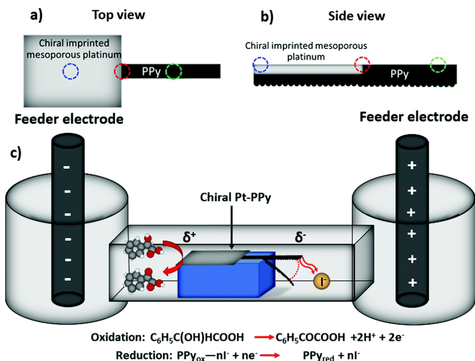
Figure 9. Schematic illustration of a hybrid bilayer composed of a free-standing conducting polymer film and a layer of mesoporous metal, encoded with chiral features (a) Top view and (b) cross section of the hybrid material (c) scheme of the bipolar electrochemical cell for the wireless optical readout of chiral information. Reproduced with permission from Ref[37]. Copyright (2019) Royal Society of Chemistry.
