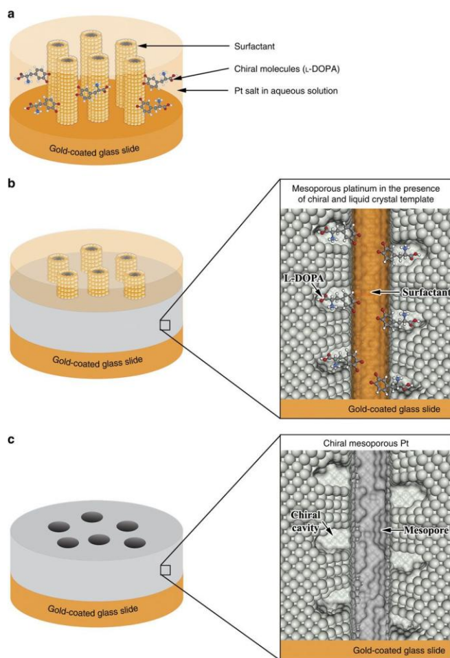
Figure 1. Schematic illustration of the preparation process of chiral imprinted mesoporous platinum in the presence of a surfactant based self-assembled lyotropic liquid crystal and chiral molecules (a) self-assembly of the lyotropic liquid crystal and the chiral template molecules; (b) electroreduction of platinum ions around the templates at a constant applied negative potential; (c) template dissolution. Reproduced with permission from Ref[12a]. Copyright (2014) Springer Nature Group.
