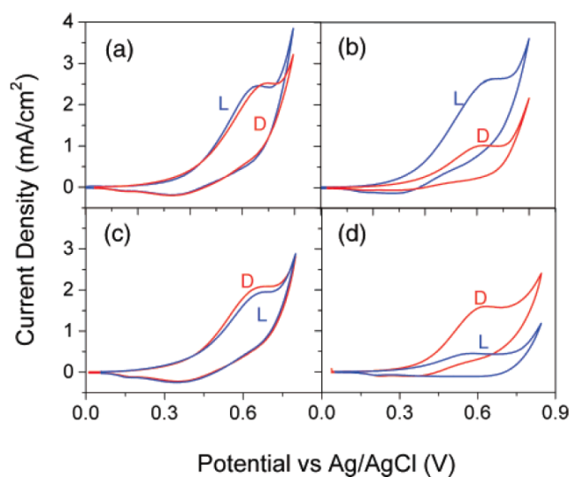
Figure 3. Illustration of the chiral recognition of tartrate ions by electrooxidation on imprinted CuO films obtained by etching with tartrate enantiomers. Cyclic voltammetry (CV) measurements in L(+)-tartrate (blue) and D(-) tartrate (red) in 1.0 M NaOH: (a) as-deposited CuO from L(+)-tartrate; (b) same film after etching in L(+)-tartaric acid; (c) as deposited CuO film from D(-)-tartrate; (d) same film after etching in D(-)-tartaric acid. Reproduced with permission from Ref[31a]. Copyright (2007) American Chemical Society.
