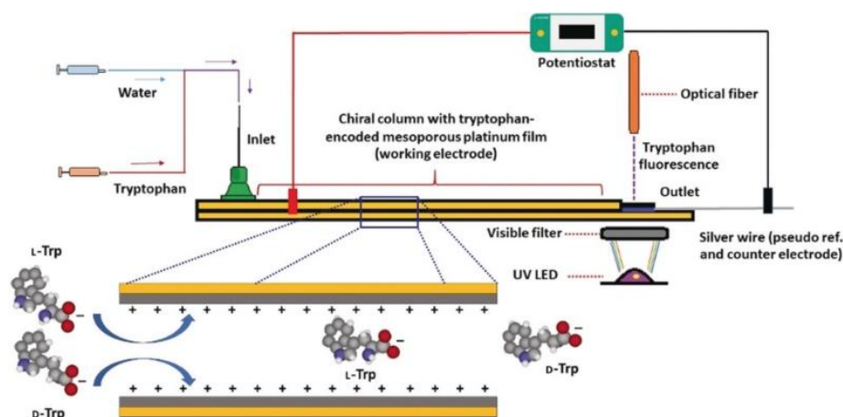
Figure 8. Schematic illustration of the concept of chiral electrochromatography. A chiral mesoporous metal imprinted with L-Tryptophan is used as a stationary phase in a microfluidic electrochromatography device. The enantioaffinity can be easily tuned by applying a suitable potential to the stationary phase controlled by a potentiostat. Reproduced with permission from Ref[20b]. Copyright (2019) Wiley-VCH Verlag GmbH & Co. KGaA, Weinheim.
