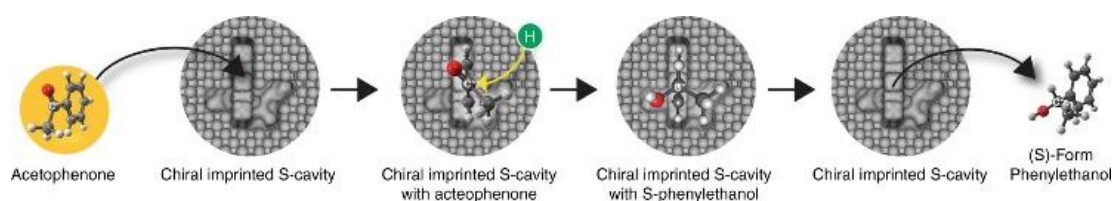
Figure 7. Schematic illustration of the pulsed electroreduction of acetophenone to phenylethanol enantiomers on molecular imprinted mesoporous platinum films including three important steps: (I) the adsorption of acetophenone in the chiral imprinted cavities of the mesoporous metal; (II) the stereoselective reduction of acetophenone to phenylethanol enantiomers; (III) the desorption of phenylethanol and the regeneration of empty chiral cavities for the next catalytic cycle. Reproduced with permission from Ref[20a]. Copyright (2017) Springer Nature Group.
