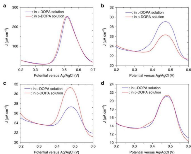
Figure 5. Chiral recognition of DOPA enantiomers revealed by differential pulse voltammetry (DPV) with molecular imprinted mesoporous platinum: (a) a flat platinum electrode; (b) a chiral mesoporous platinum electrode imprinted with L-DOPA; (c) a chiral mesoporous platinum electrode imprinted with D-DOPA; (d) chiral mesoporous platinum electrodes imprinted with L-DOPA after complete destruction of the chiral information by scanning the potential between -0.2 V to 1.25 V (vs Ag/AgCl) in 0.5 M \text{H}_2\text{SO}_4 . Reproduced with permission from Ref[12a]. Copyright (2014) Springer Nature Group.
