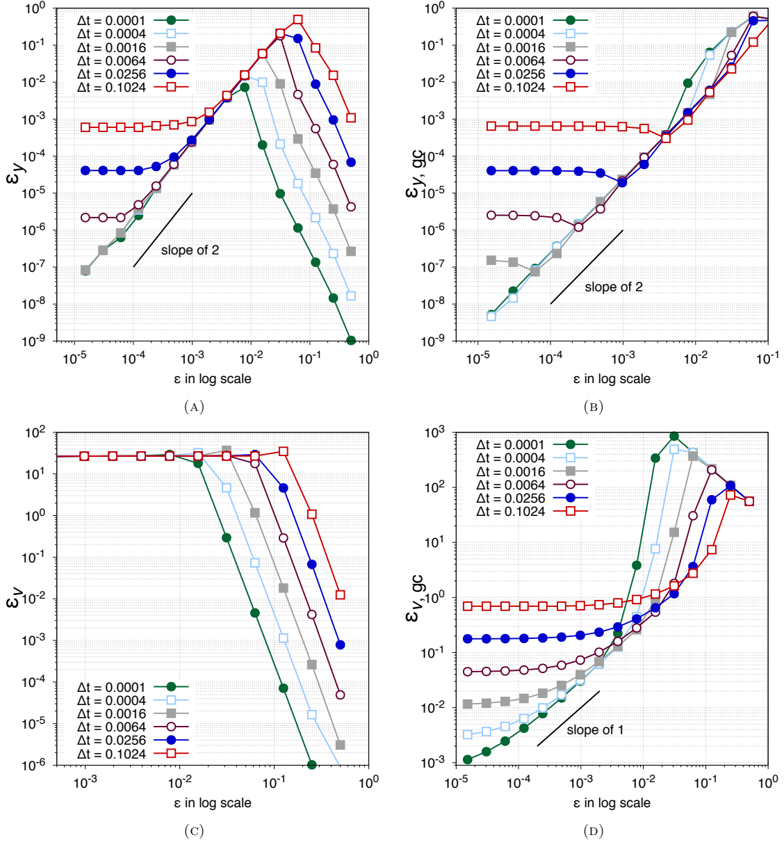
FIGURE 2. Second-order scheme (5.2) : (A) Error between the approximation \mathbf{y}_\epsilon^n and (reference) solution \mathbf{y}_\epsilon(t_n) of (1.7) denoted by \mathcal{E}_y . (B) Error between the approximation \mathbf{y}_\epsilon^n and the asymptotic (reference) solution \mathbf{X}(t_n, 0, \mathbf{x}^0 - \epsilon(\mathbf{v}^0)^\perp) of (2.1) denoted by \mathcal{E}_{y,gc} . (C) Error between the approximation \mathbf{v}_\epsilon^n and the (reference) solution \mathbf{v}_\epsilon(t_n) of (1.7) denoted by \mathcal{E}_v . (D) Error between the approximation \epsilon^{-1}\mathbf{v}_\epsilon^n and the asymptotic (reference) velocity \mathbf{v}_{gc}(t_n) denoted by \mathcal{E}_{v,gc} .
